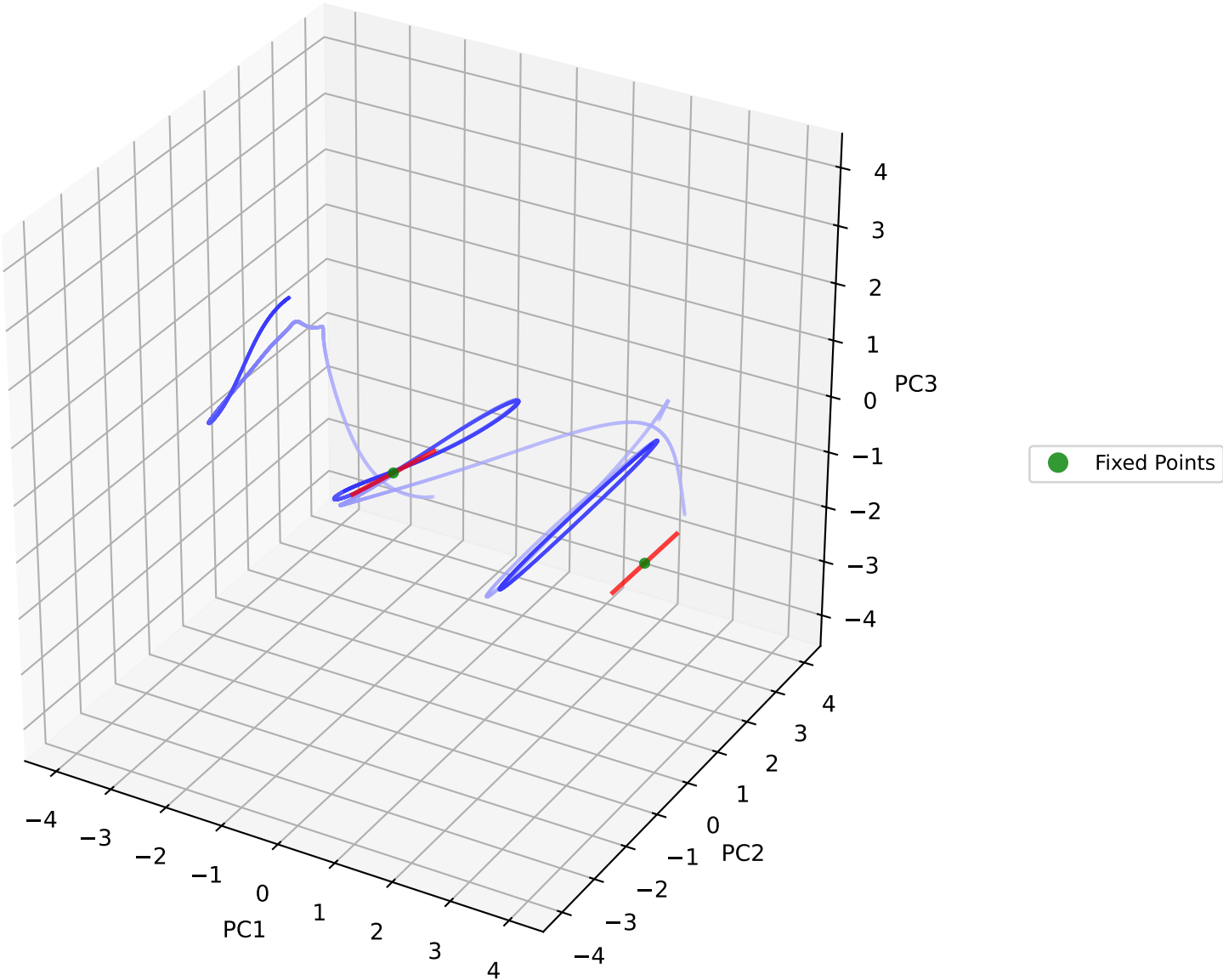
PCA of Network Trajectories and Fixed Points (tanh transformed) (Sparsity=0.00)
