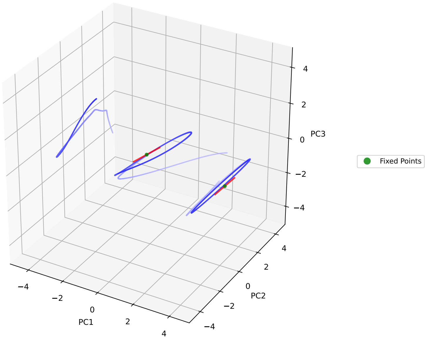
PCA of Network Trajectories and Fixed Points (skipping first 200 steps) (Sparsity=0.00)
