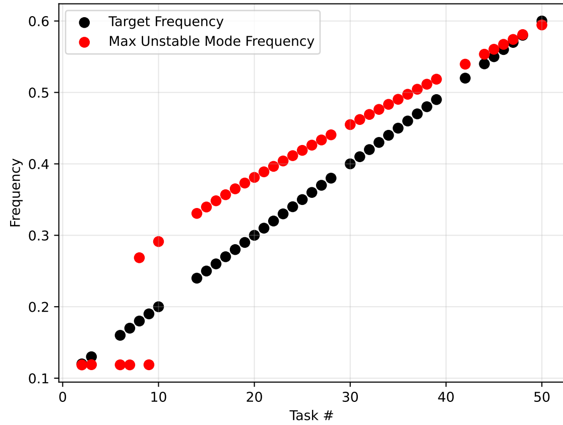
Sparsity s = 0.60 Final loss: 1.42\text{e-}04
