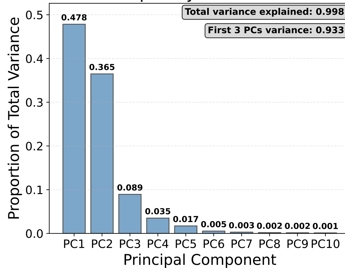
Sparsity s = 0.80
