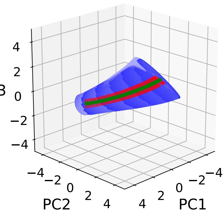
Sparsity s = 0.00
