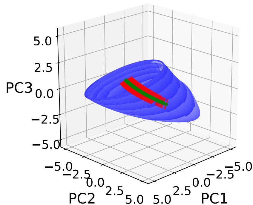
Sparsity s = 0.20
