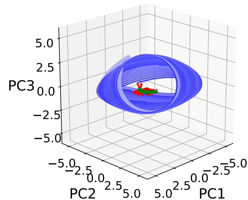
Sparsity s = 0.40
