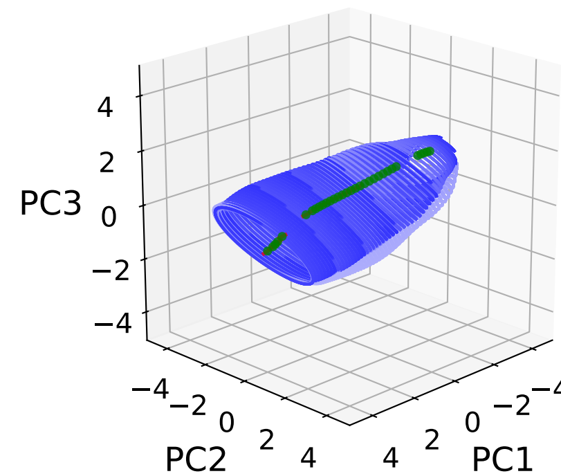
Sparsity s = 0.99
