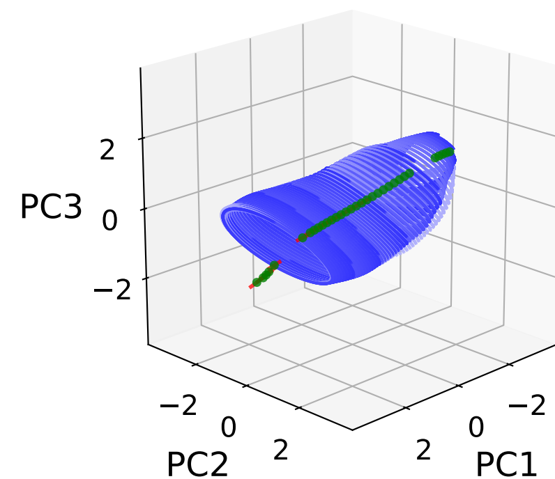
Sparsity s = 0.99
