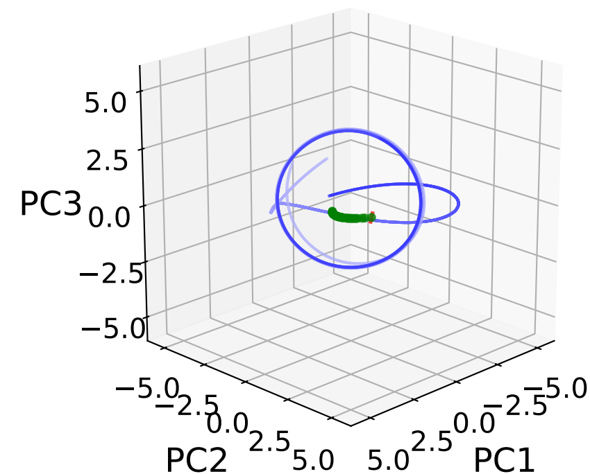
Sparsity s = 0.40
