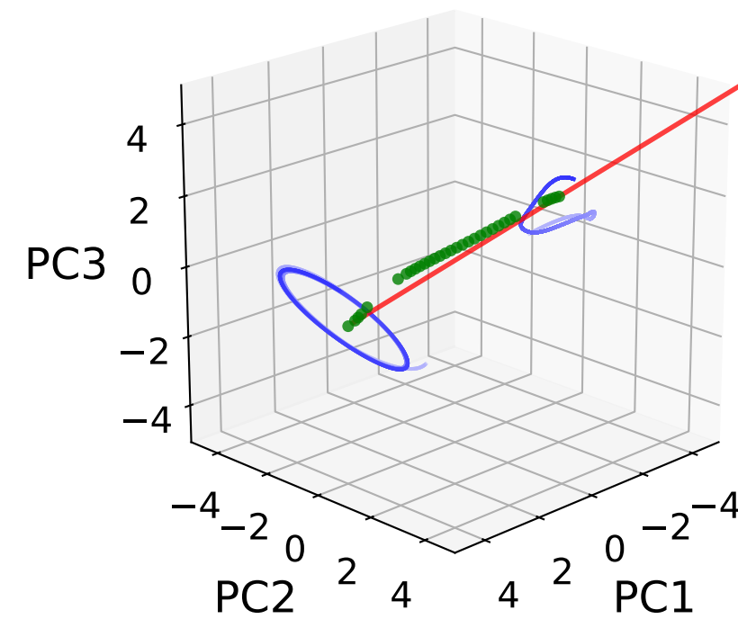
Sparsity s = 0.99
