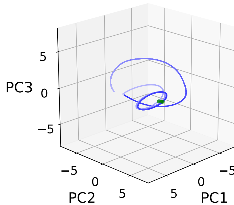
Sparsity s = 0.80
