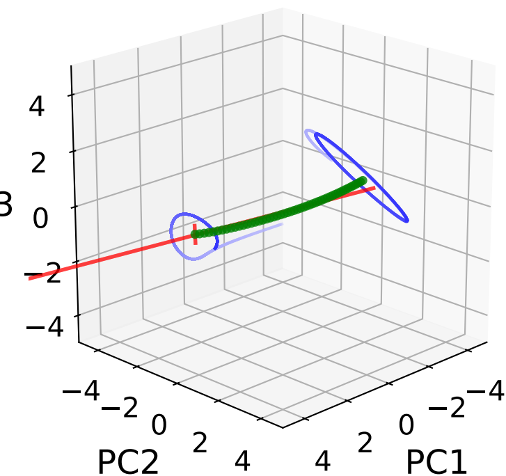
Sparsity s = 0.00
