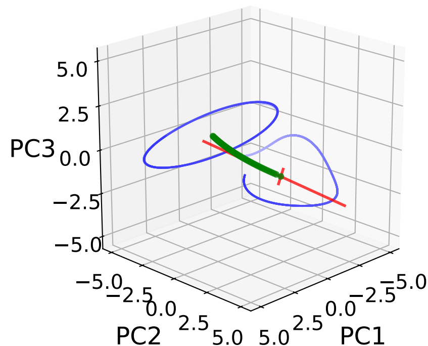
Sparsity s = 0.20
