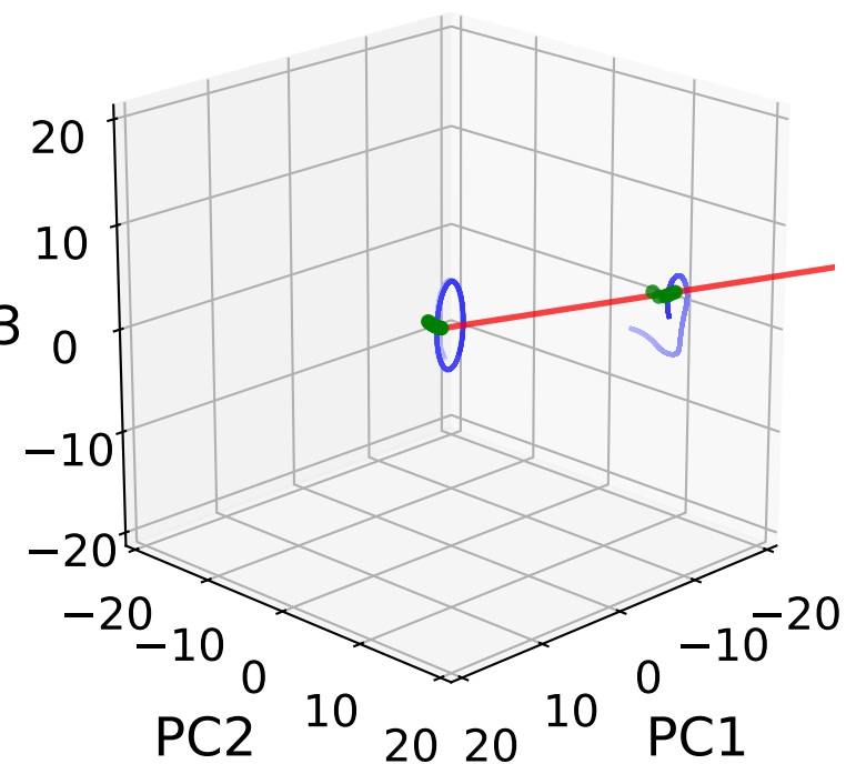
Sparsity s = 0.60
