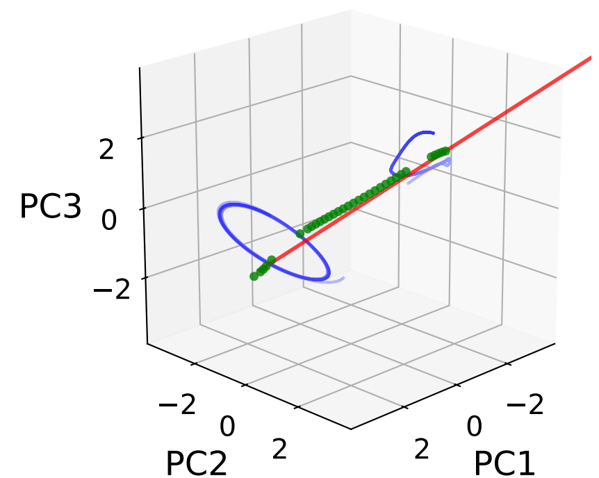
Sparsity s = 0.99
