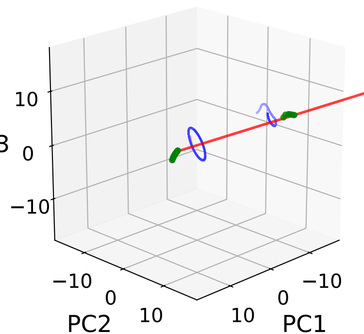
Sparsity s = 0.60
