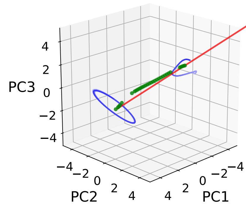
Sparsity s = 0.99
