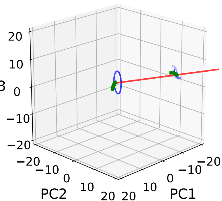
Sparsity s = 0.60
