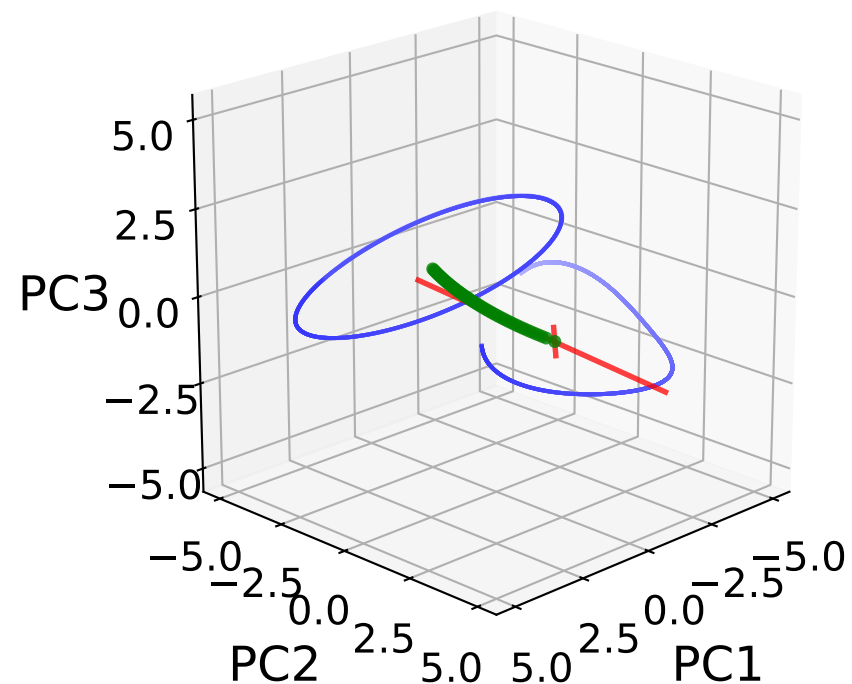
Sparsity s = 0.20
