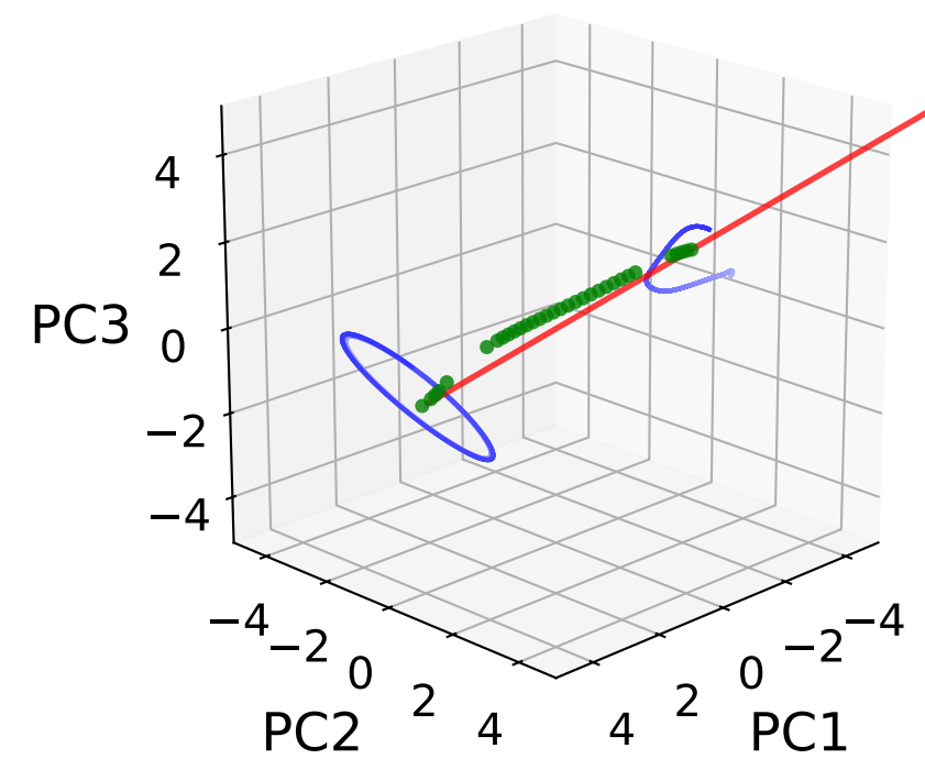
Sparsity s = 0.99
