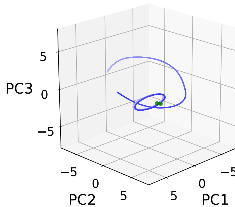
Sparsity s = 0.80
