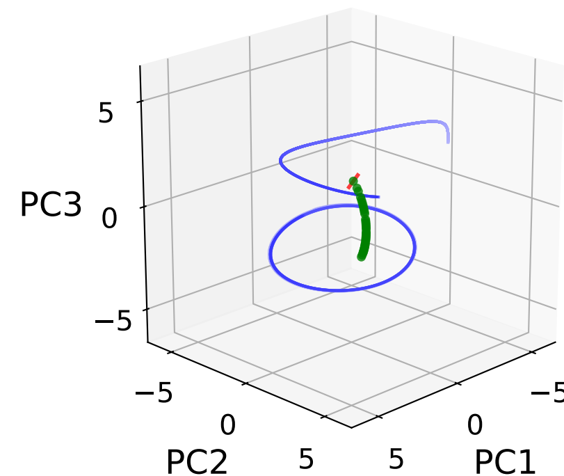
Sparsity s = 0.40
