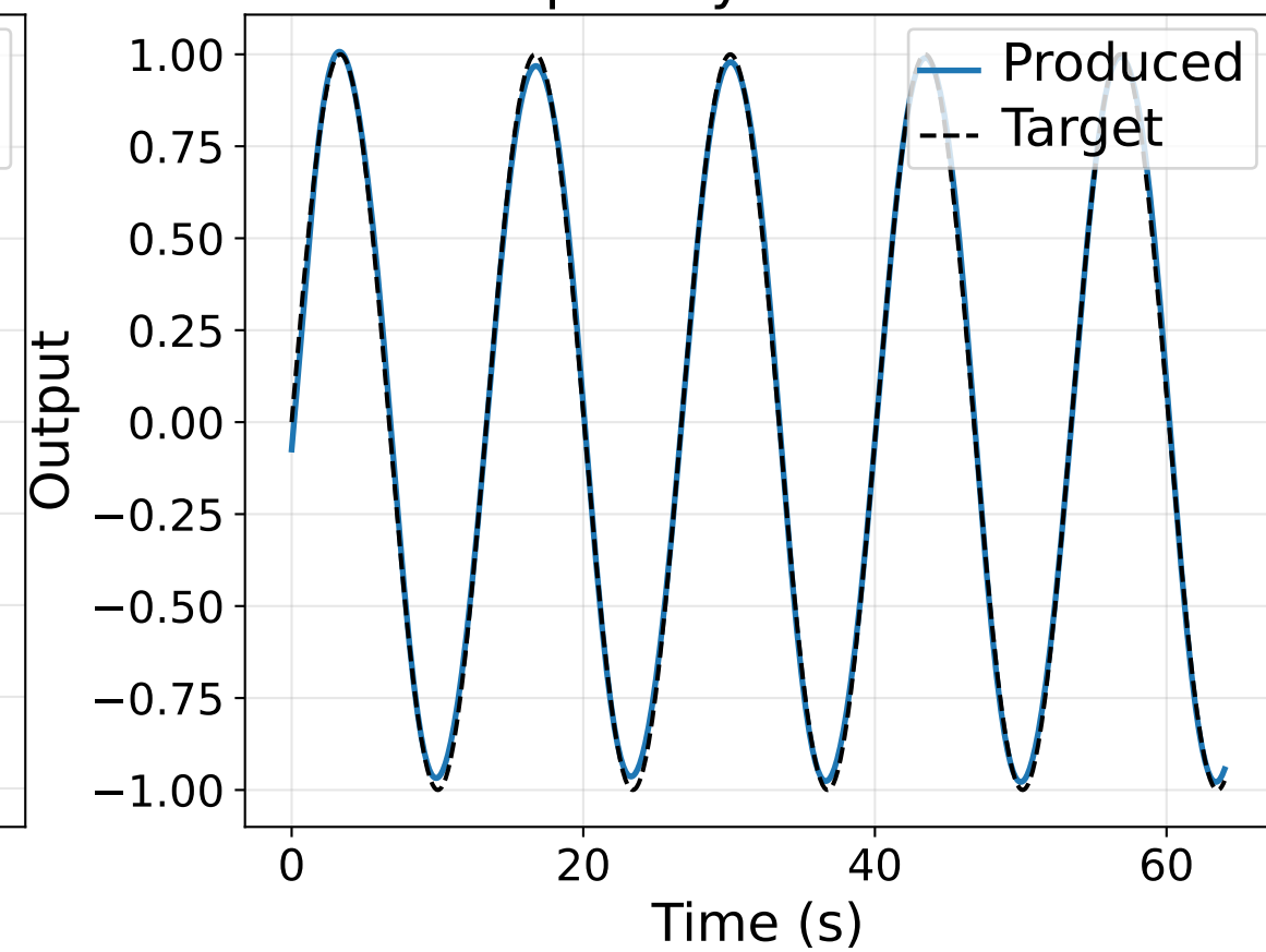
Sparsity s = 0.99
