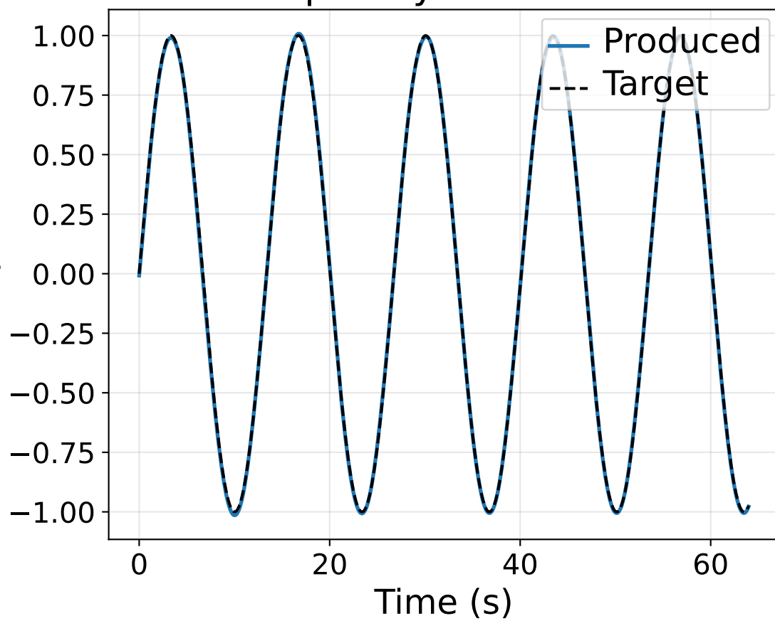
Sparsity s = 0.60
