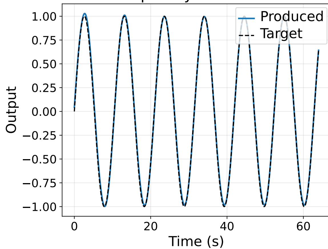
Sparsity s = 0.60
