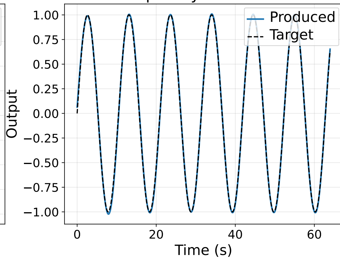
Sparsity s = 0.80
