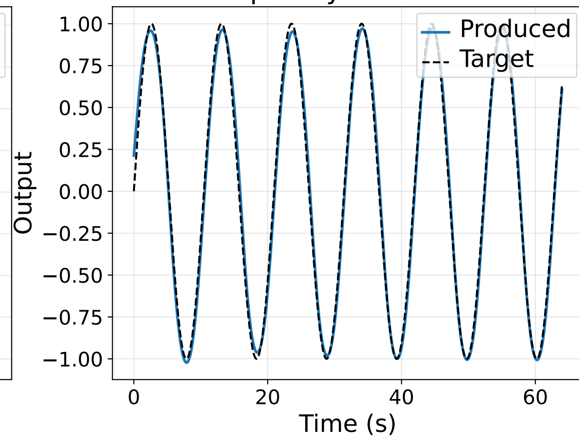
Sparsity s = 0.99
