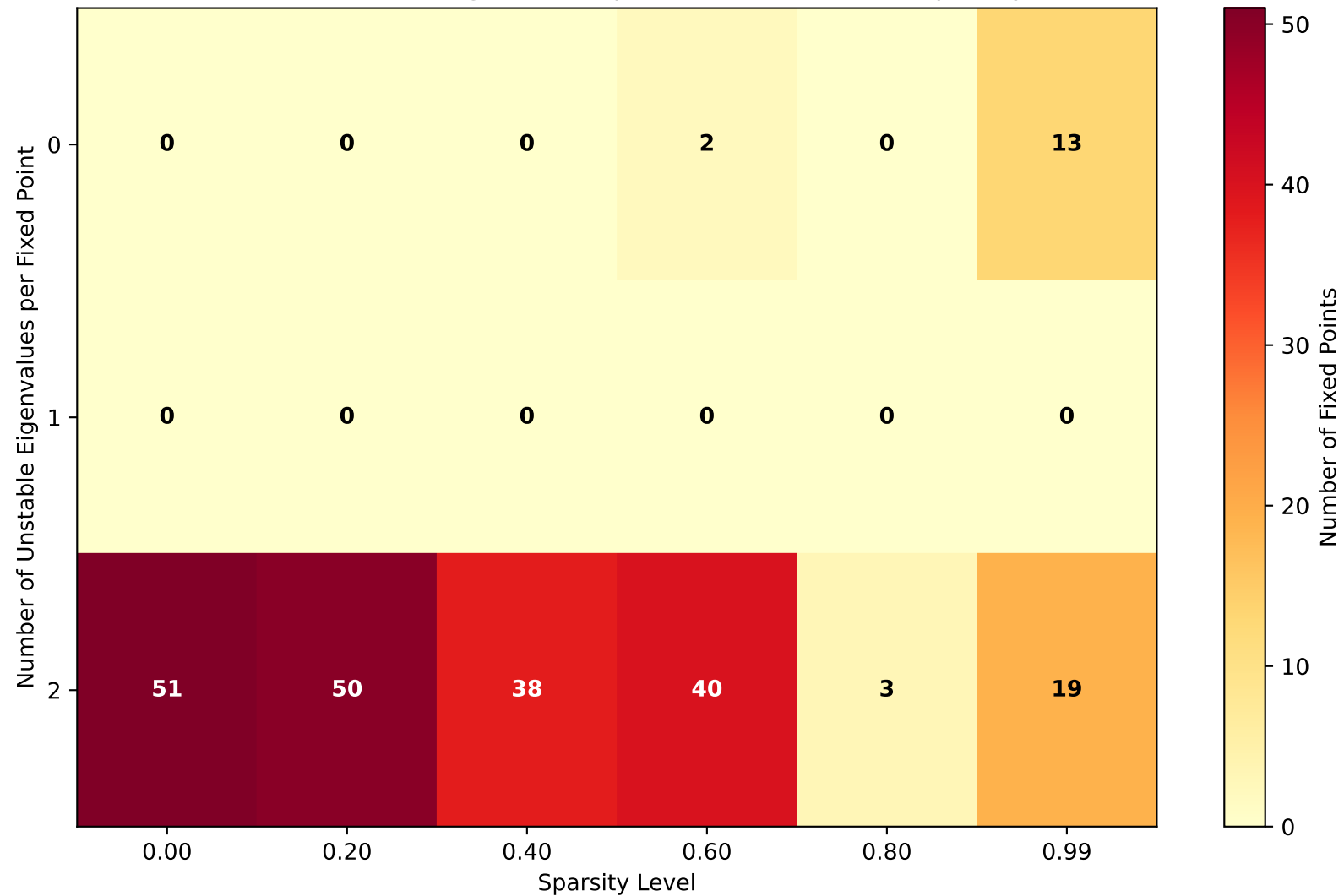
Distribution of Unstable Eigenvalues per Fixed Point Across Sparsity Levels
