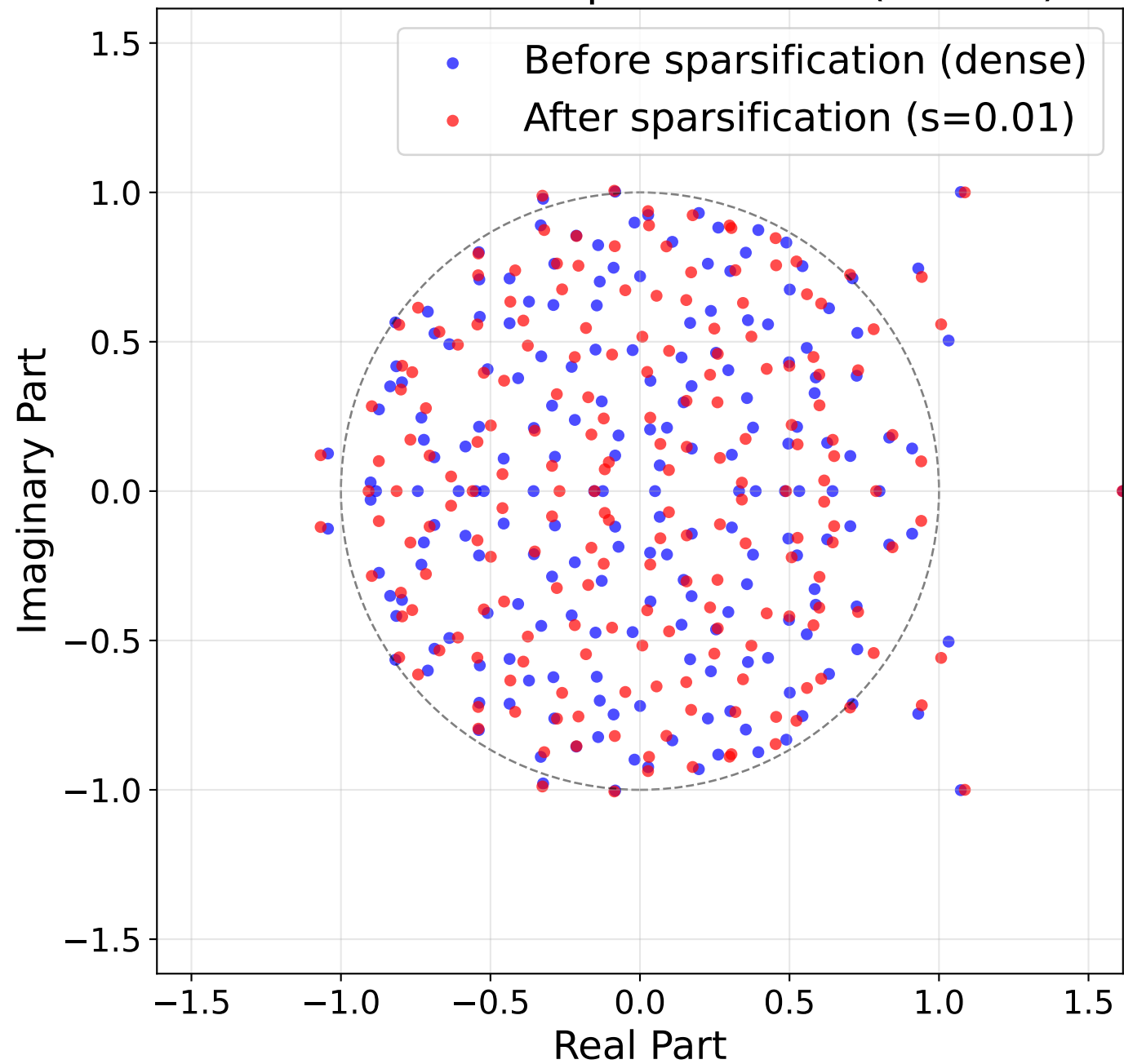
Connectivity Matrix Eigenvalues Before vs After Sparsification ( s=0.01 )
