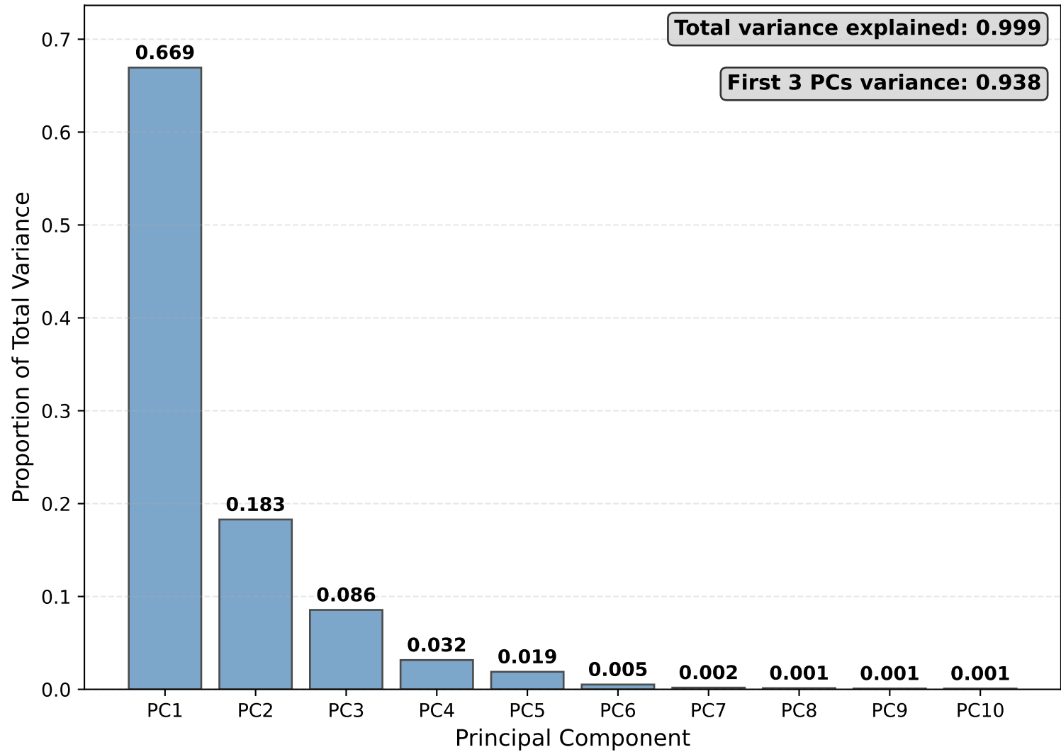
PCA Explained Variance Ratio (skipping first 200 steps) (tanh transformed) (Sparsity=0.00)
