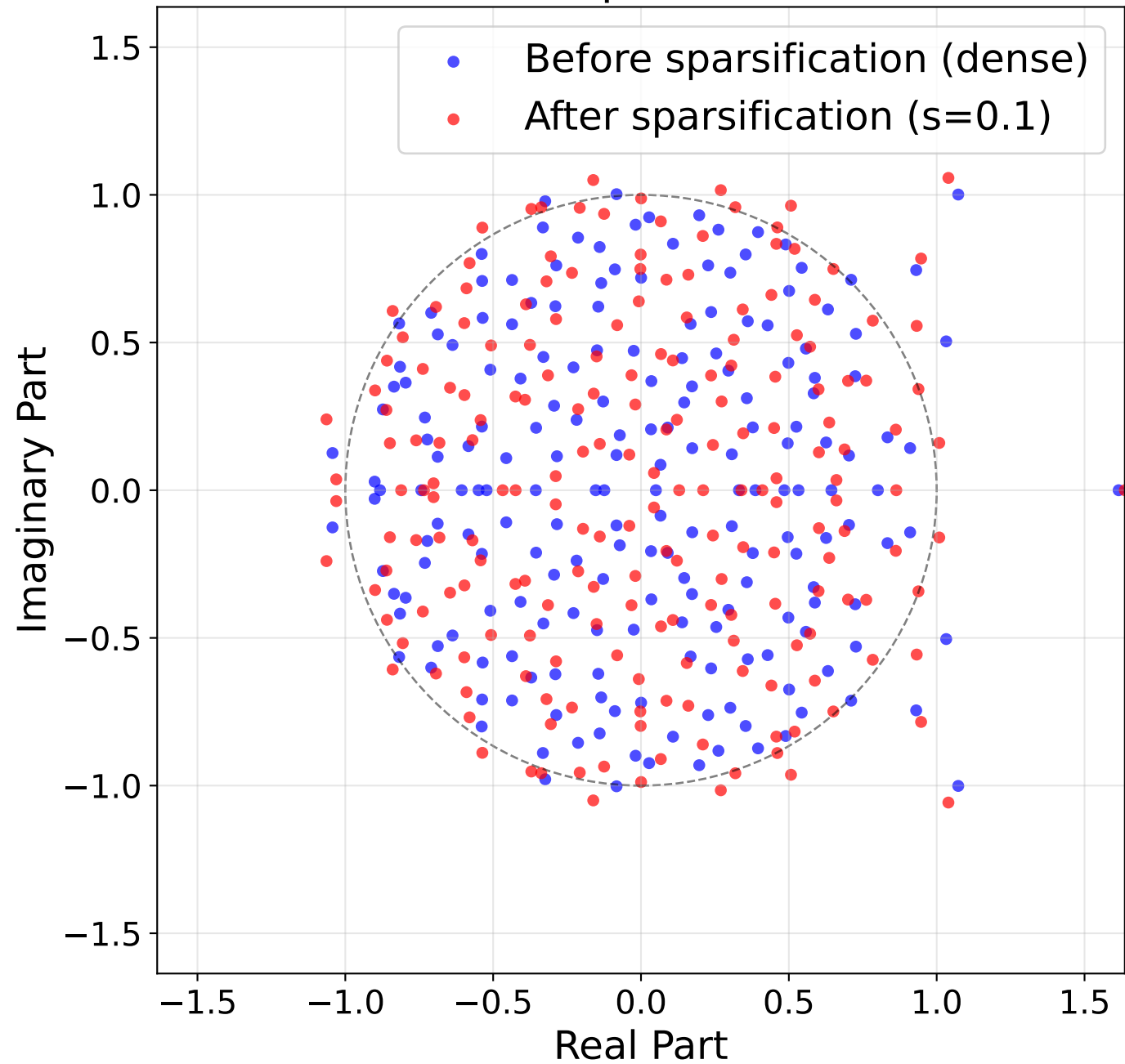
Connectivity Matrix Eigenvalues Before vs After Sparsification ( s=0.1 )
