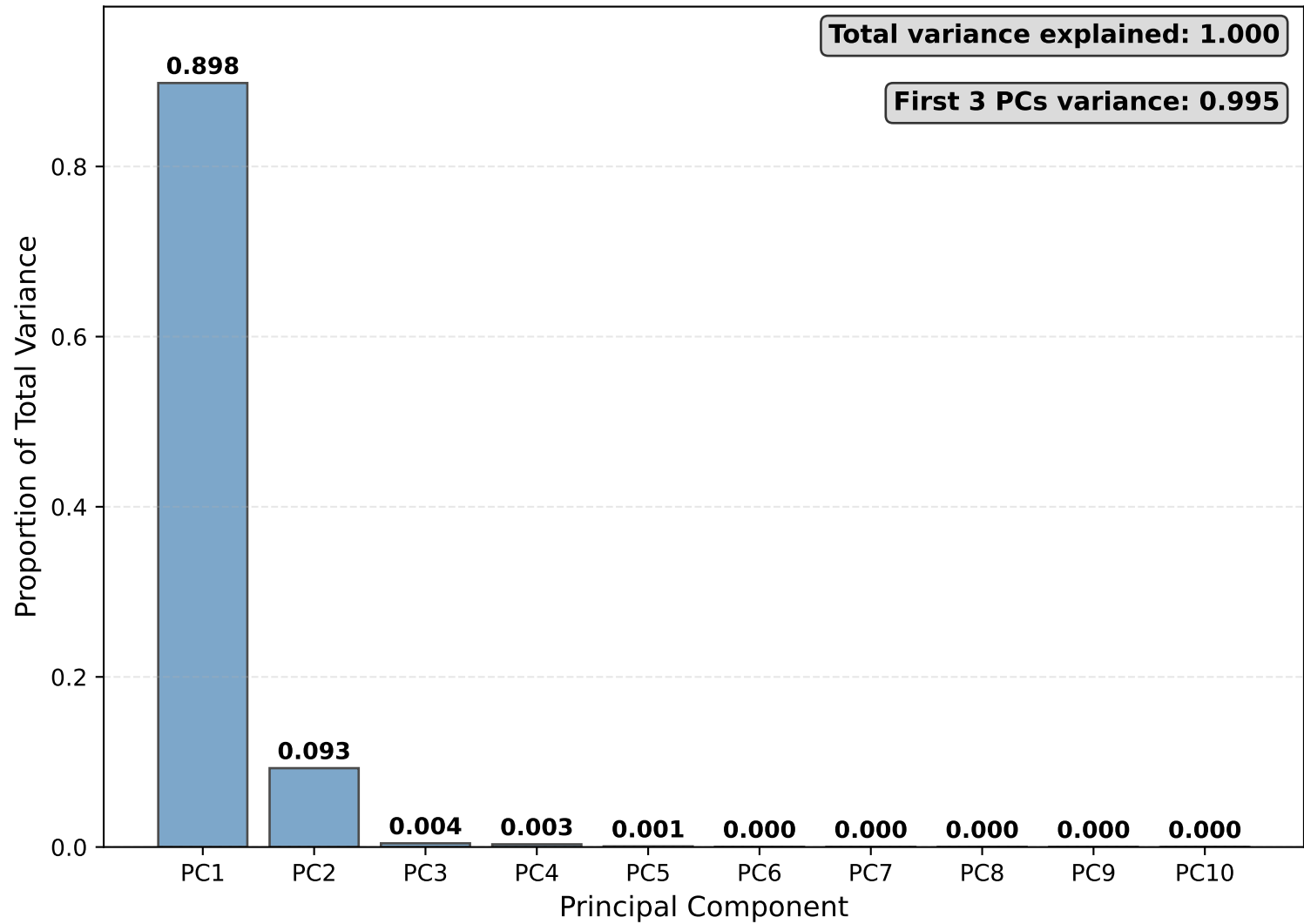
PCA Explained Variance Ratio (skipping first 600 steps) (tanh transformed) (Sparsity=0.00)
