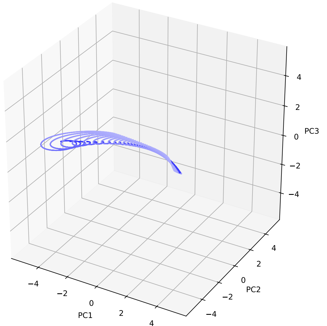
PCA of Network Trajectories and Fixed Points (skipping first 600 steps) (Sparsity=0.00)
