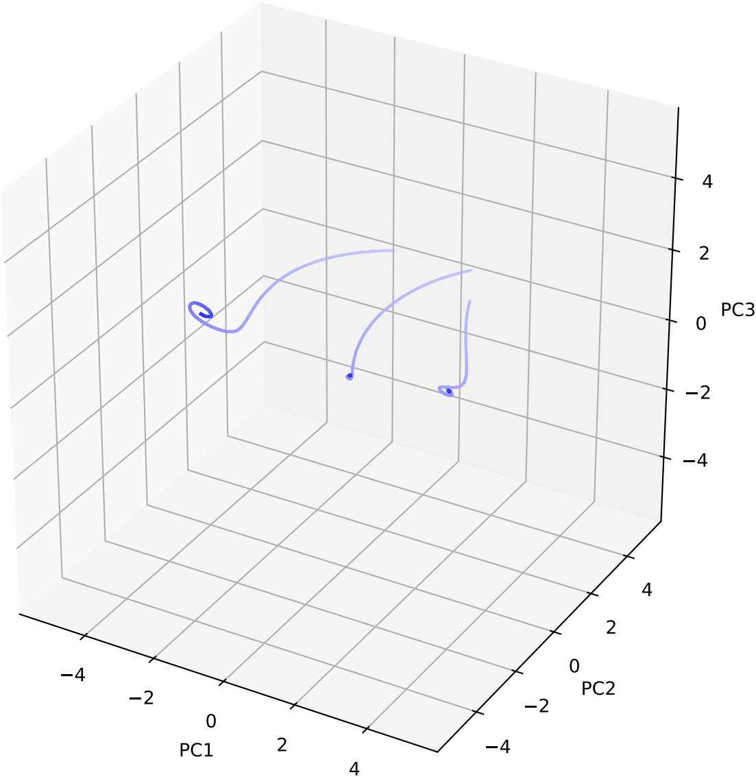
PCA of Network Trajectories and Fixed Points (skipping first 200 steps) (Sparsity=0.00)
