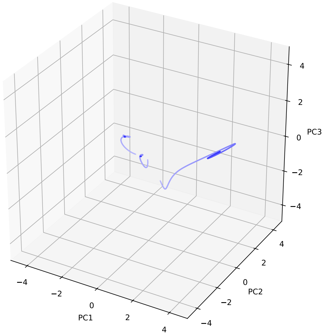
PCA of Network Trajectories and Fixed Points (skipping first 200 steps) (tanh transformed) (Sparsity=0.00)
