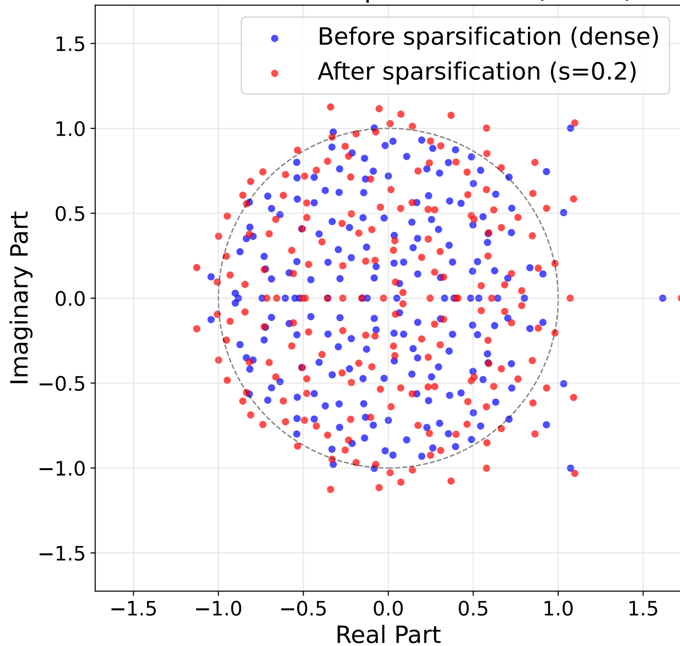
Connectivity Matrix Eigenvalues Before vs After Sparsification ( s=0.2 )
