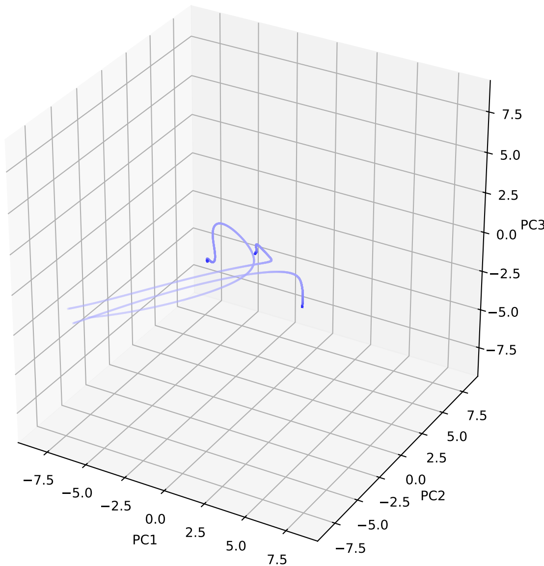
PCA of Network Trajectories and Fixed Points (Sparsity=0.00)
