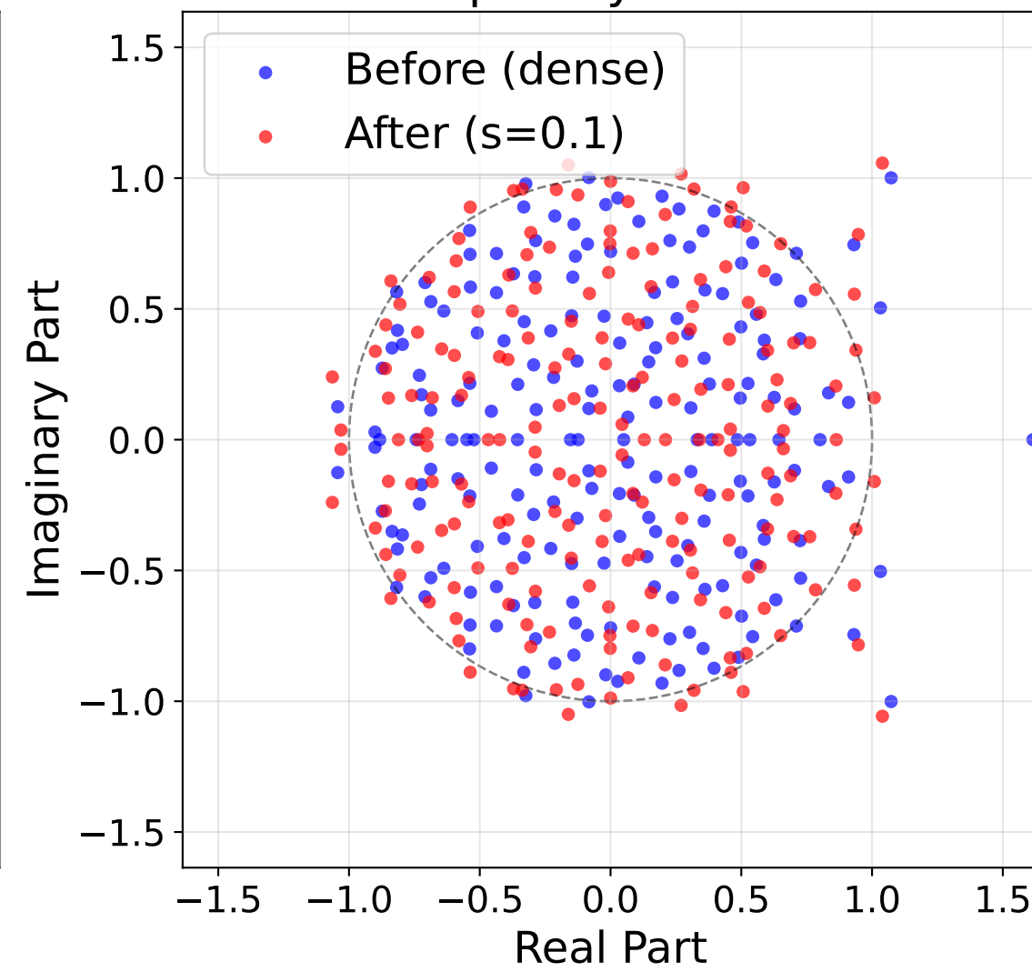
Sparsity = 0.1
