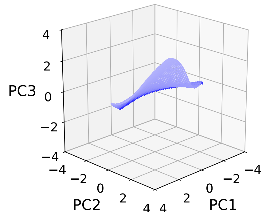
Sparsity s = 0.20
