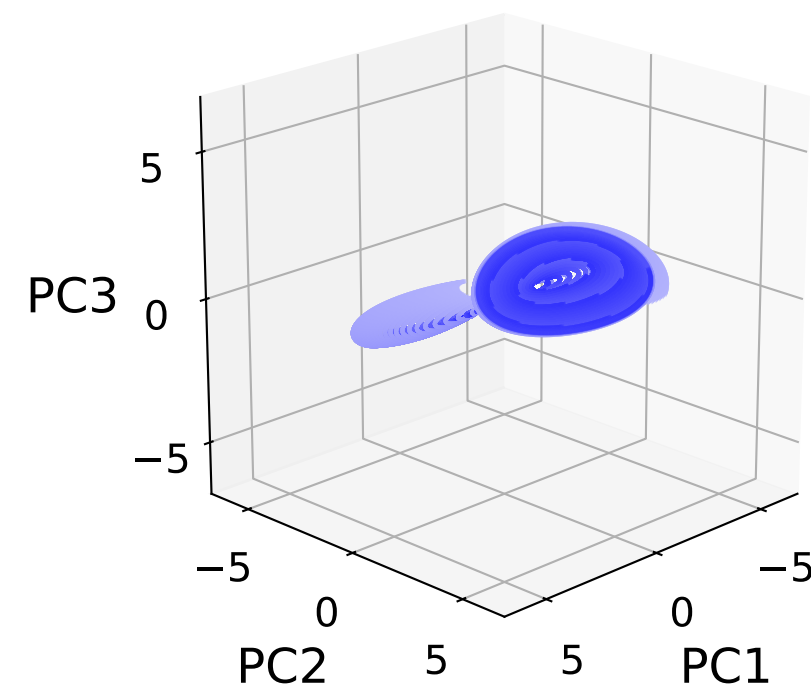
Sparsity s = 0.02
