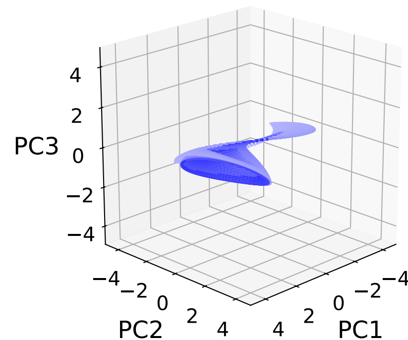
Sparsity s = 0.02
