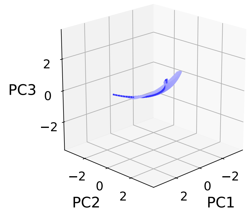
Sparsity s = 0.20
