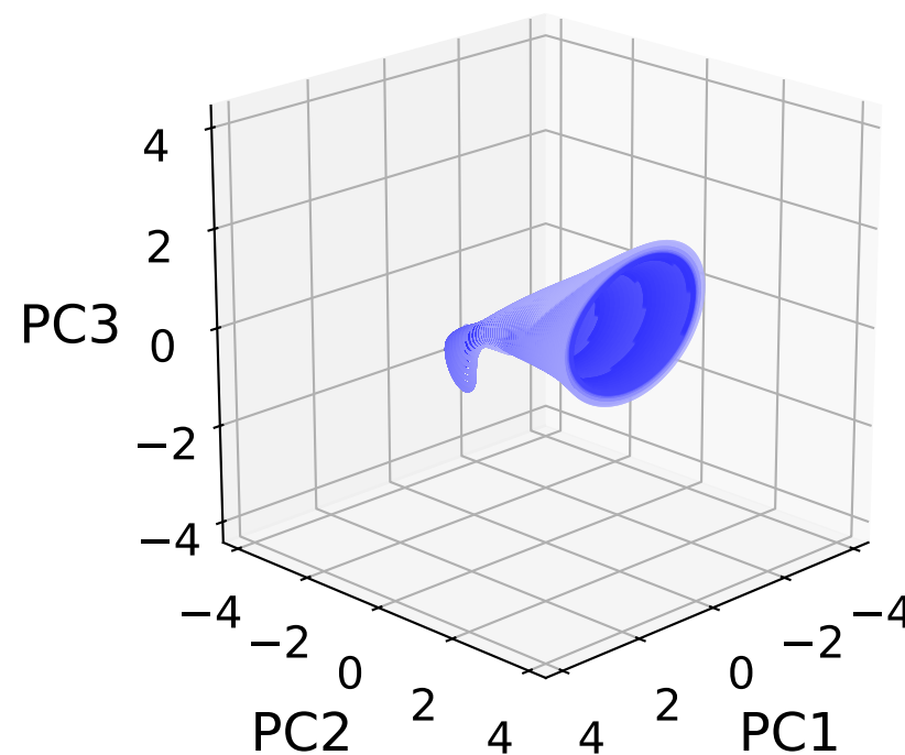
Sparsity s = 0.01
