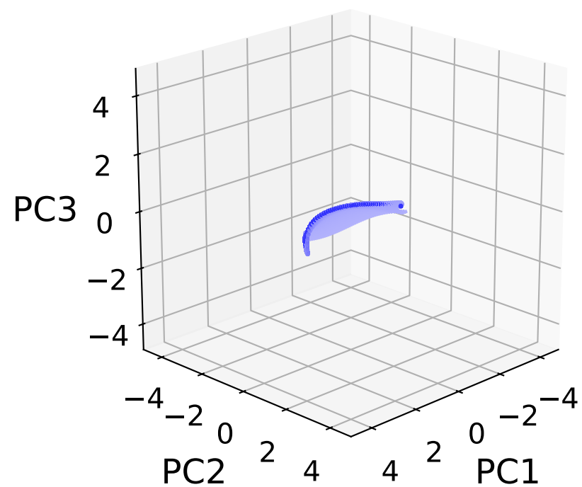
Sparsity s = 0.10
