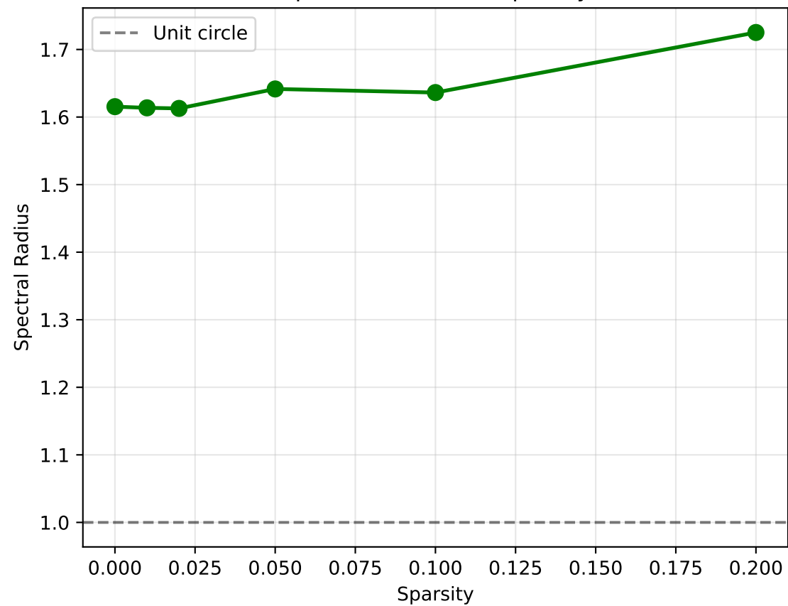
Spectral Radius vs Sparsity
