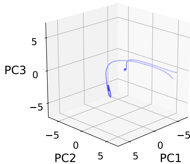
Sparsity s = 0.10
