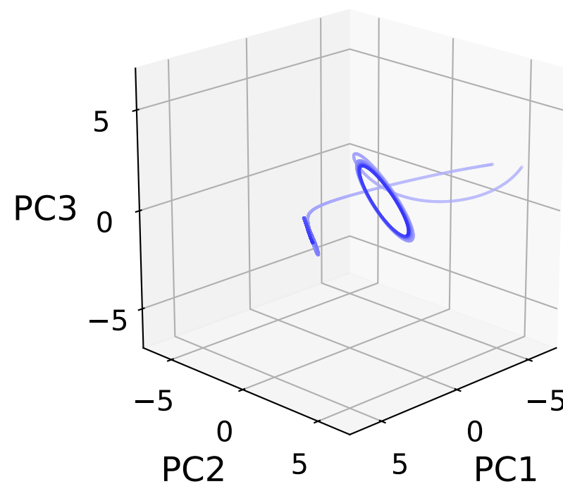
Sparsity s = 0.01
