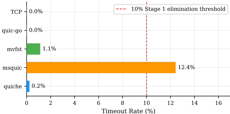
Timeout Rate per Implementation (43,200 conditions each)
