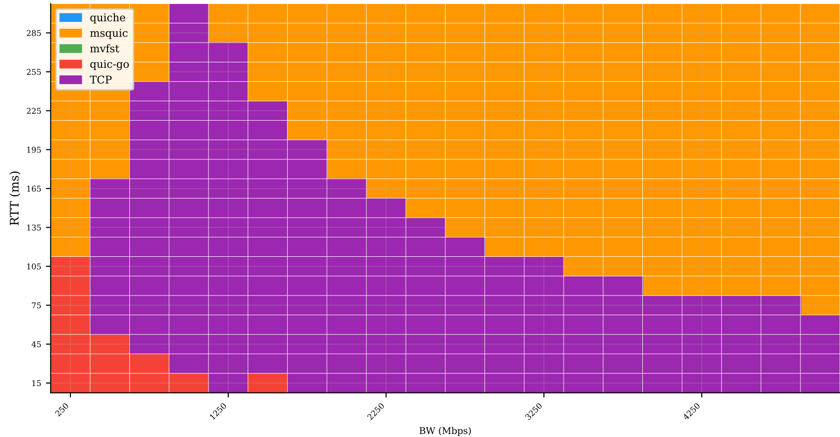
Implementation with Highest Raw Goodput per (Bandwidth, RTT) — clean, no impairments
