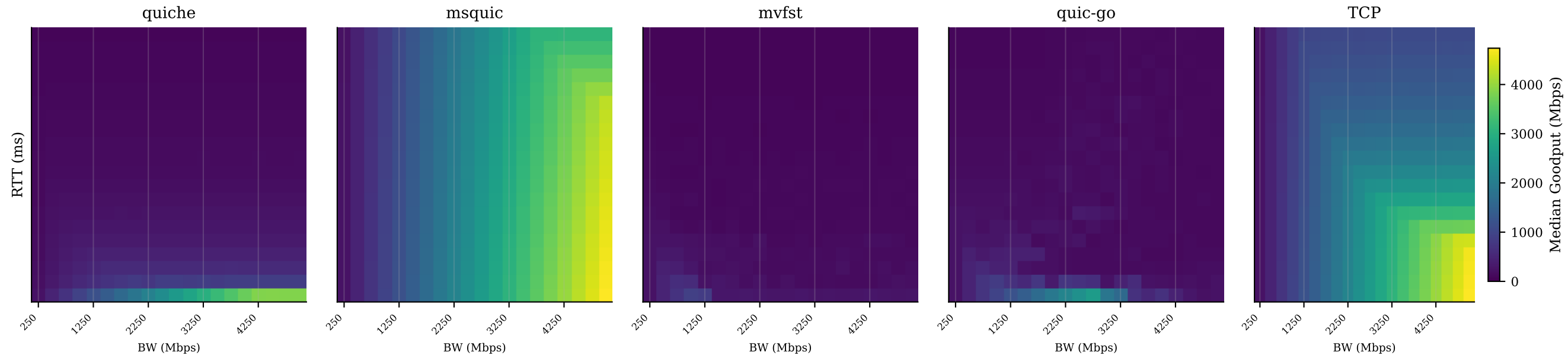
Goodput Heatmap per Implementation (clean condition)
