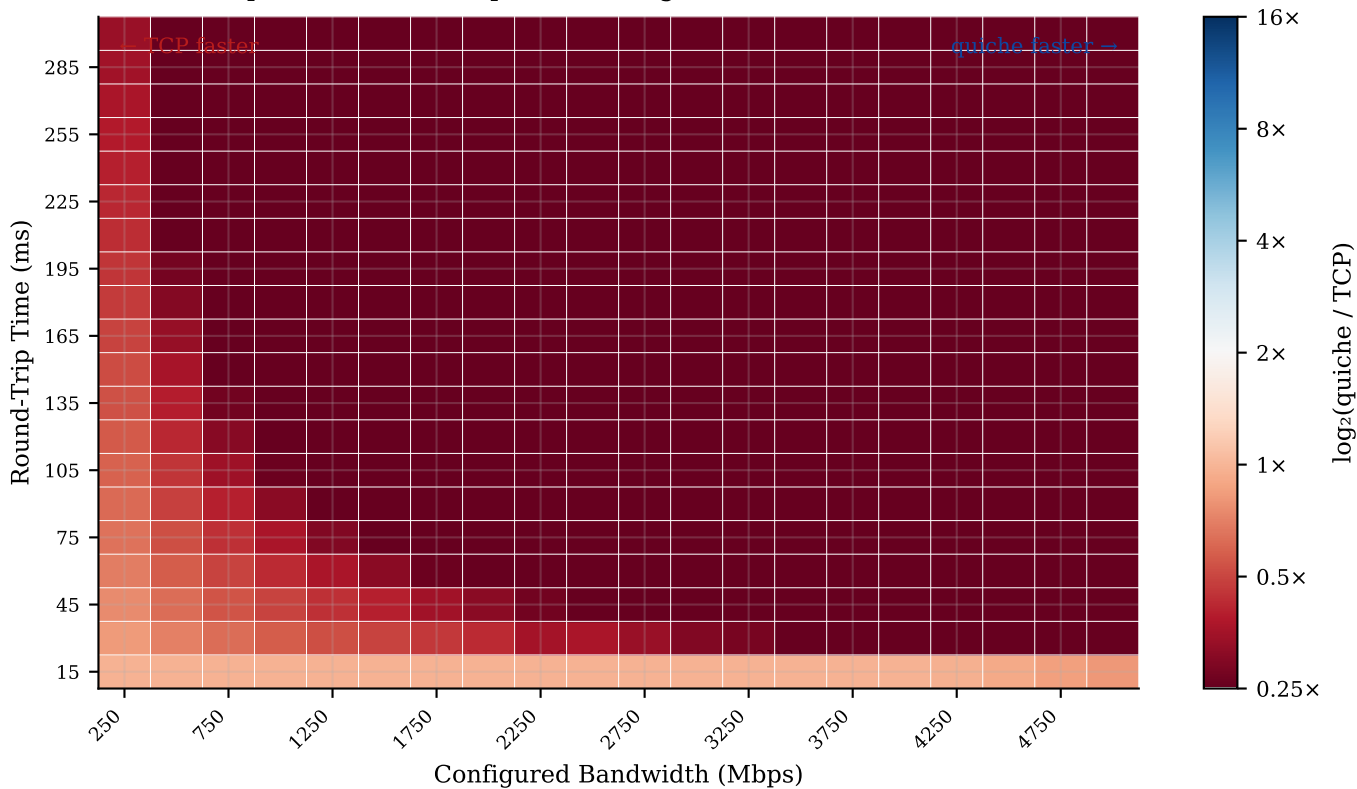
quiche / TCP Goodput Ratio (log 2 scale, clean condition)
