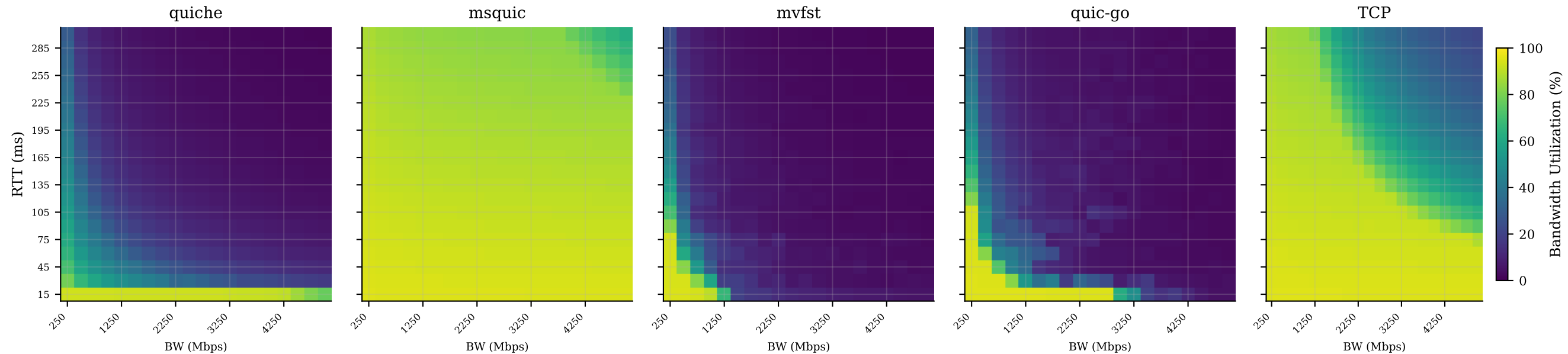
Bandwidth Utilization: Goodput / Configured Bandwidth (clean condition)
