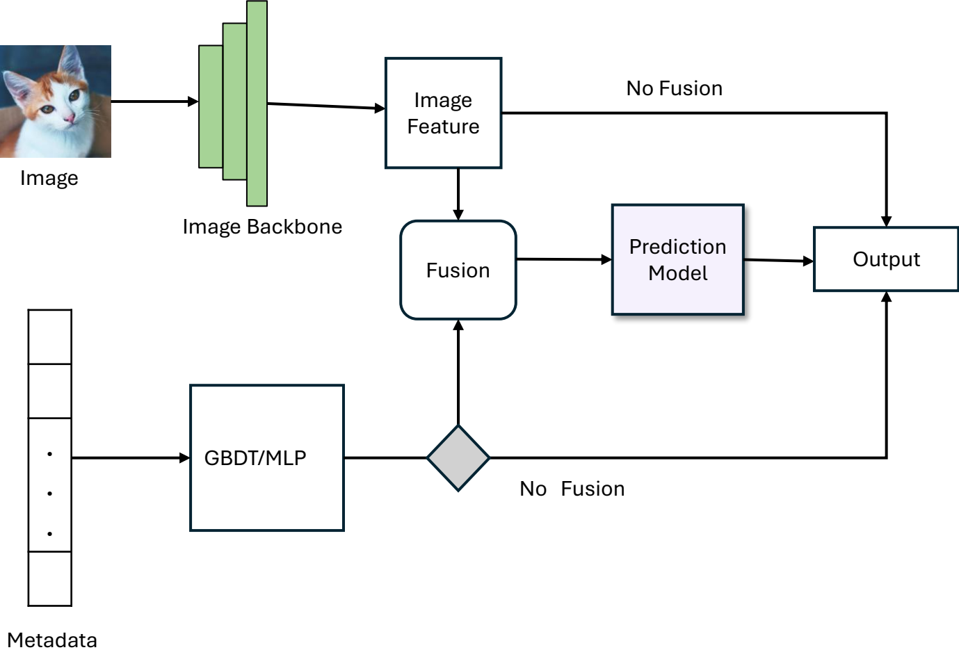
Figure 1: Pipeline
