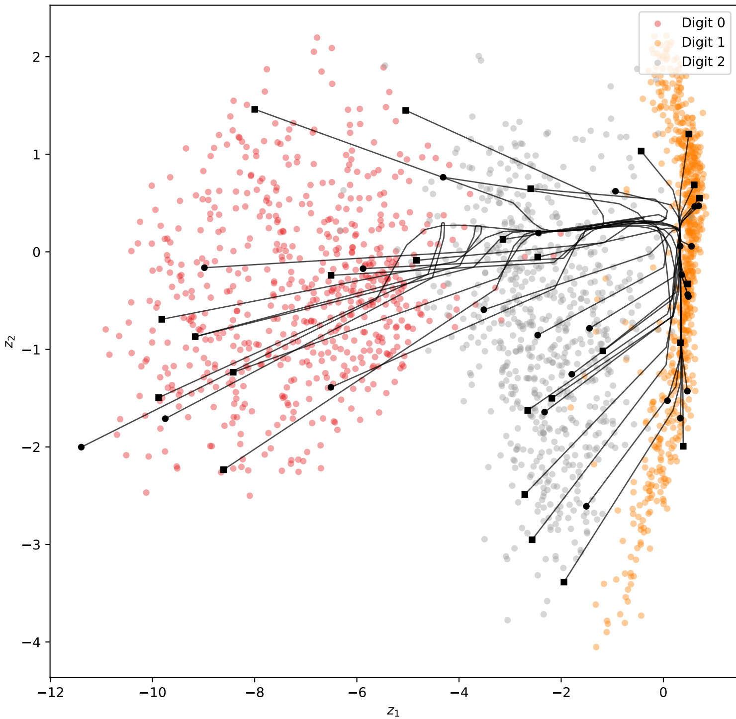
Geodesics (K=3 decoders)
