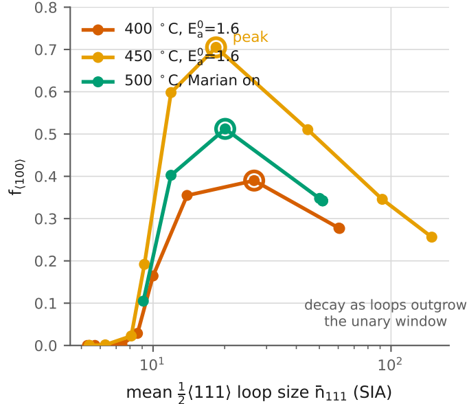
(b) Transient: unary alone cannot hold large loops
