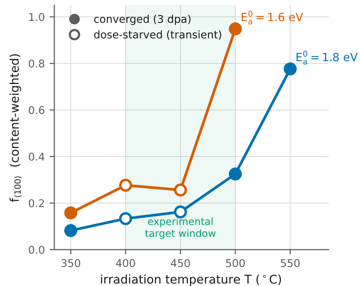
(a) Loop-character fraction vs temperature
