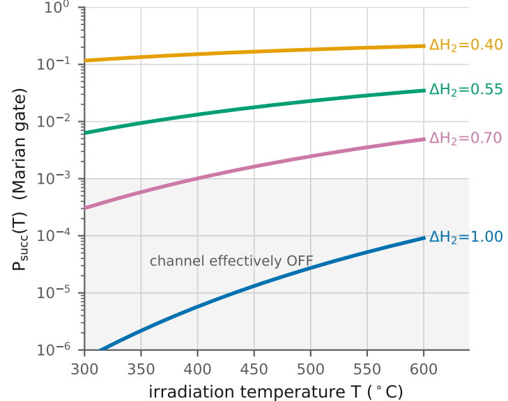
(c) Marian gate: magnitude vs. T-sensitivity
