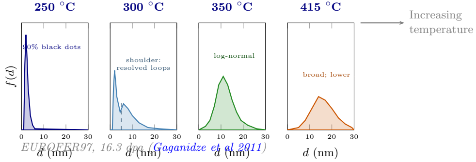
Fig. 12 Schematic representation of the temperature-dependent evolution of dislocation loop size distributions in EUROFER97 (16.3 dpa, BOR-60 neutron irradiation). At 250 °C, the distribution is dominated by a narrow spike of sub-3 nm black-dot defects ( \sim 90\% ). At 300 °C, a resolved-loop shoulder develops at 5–15 nm while the black-dot peak persists. Above 350 °C, the distribution becomes a well-developed log-normal centred at 10–13 nm. At 415 °C, the distribution broadens further and the total density decreases as large loops begin transforming into network dislocations.
