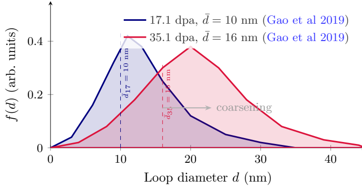
Fig. 13 Schematic dose evolution of the dislocation loop size distribution in HT9 at 377 °C (BOR-60 neutron irradiation). The distribution shifts rightward and the peak height decreases, indicative of coarsening: mean diameter increases from \sim 10 nm at 17.1 dpa to \sim 16 nm at 35.1 dpa while total loop number density decreases (Gao et al 2019).
