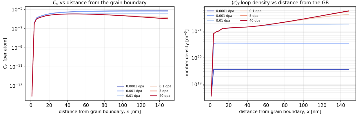
Figure 13: Profiles against distance from the boundary over the first 150 nm, with every dose overlaid. Left: the mobile vacancy concentration, whose recovery length is the boundary layer tabulated above and which narrows as the dose accumulates. Right: the basal \langle c \rangle loop number density, whose profile is the denuded zone of Fig. 12 seen at every dose rather than only at the last.
