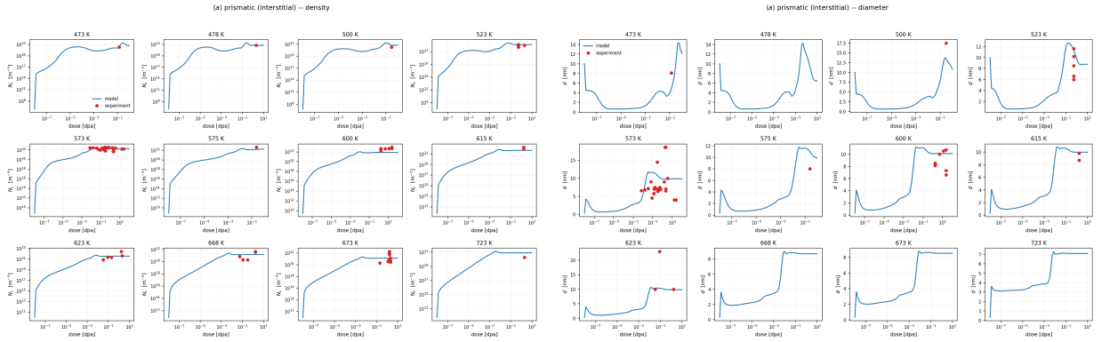
Figure 3: Prismatic \langle a \rangle loops by temperature: number density (left) and mean diameter (right), 71 and 44 points.
