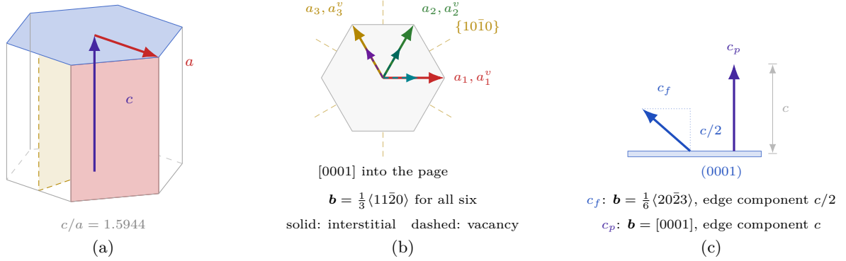
Figure 1: The hcp cell of \alpha -Zr and every Burgers vector the model carries, drawn at the physical axial ratio c/a = 1.5944 rather than the ideal \sqrt{8/3} = 1.6330 . (a) The cell, with the three planes that matter: the basal (0001) plane (blue), the habit of c_0 , c_f and c_p ; a first-order prismatic \{10\bar{1}0\} face (red), a side face of the prism; and a second-order \{11\bar{2}0\} plane (yellow, dashed), a diagonal through the cell rather than a face of it. The arrows are the two shortest lattice translations, a = \frac{1}{3}\langle 11\bar{2}0 \rangle in the basal plane and c = [0001] along the cell axis. (b) Plan view down [0001] : the three prismatic variants at 60^\circ to one another, each drawn twice — long and solid for the interstitial family, short and dashed for its vacancy partner, which shares the habit plane and the Burgers vector and differs only in what it stores. The dashed yellow lines are the \{10\bar{1}0\} traces, which bisect the Burgers directions. (c) The basal pair, seen edge-on. The perfect state c_p has \mathbf{b} = [0001] normal to its habit, so its edge component is the full c ; the faulted state c_f has the inclined \mathbf{b} = \frac{1}{6}\langle 20\bar{2}3 \rangle , whose edge component is c/2 — one removed basal layer against two. That factor of two is why \lambda_{c_p} = \lambda_{c_f}/\sqrt{2} in Table 1, and it is why the axial ratio has to be drawn correctly. The pyramid c_0 has no Burgers vector and so appears in neither panel. The inclined pyramidal planes containing \langle c+a \rangle = \frac{1}{3}\langle 11\bar{2}3 \rangle carry no family: that vector is the glide vector accommodating c -axis strain in deformation, and its planes are not observed habit planes for irradiation-induced loops, so the absence is an experimental statement and not a truncation.
