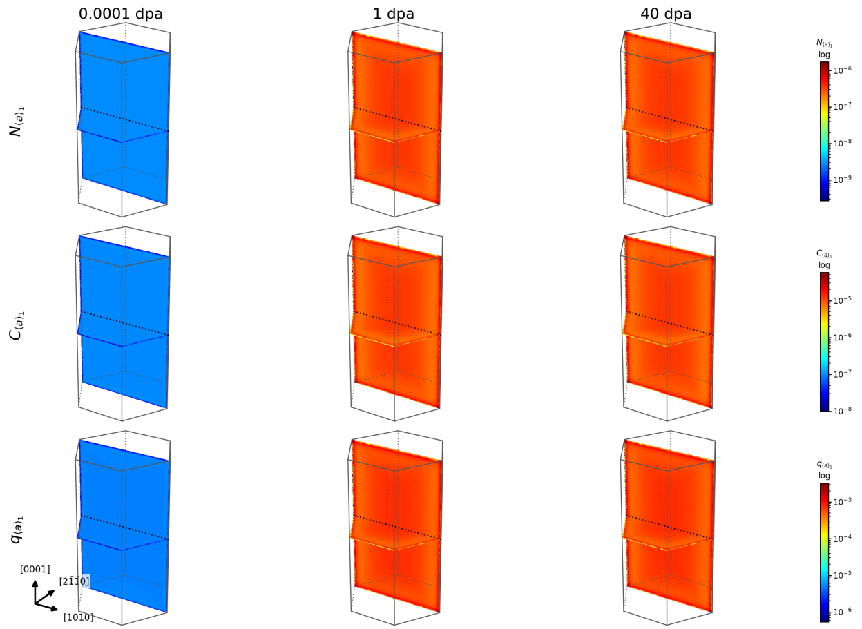
Figure 9: The prismatic interstitial variant a_1 at the same three doses, same three moments. The variants a_2 and a_3 are identical at zero applied stress and are not shown.
