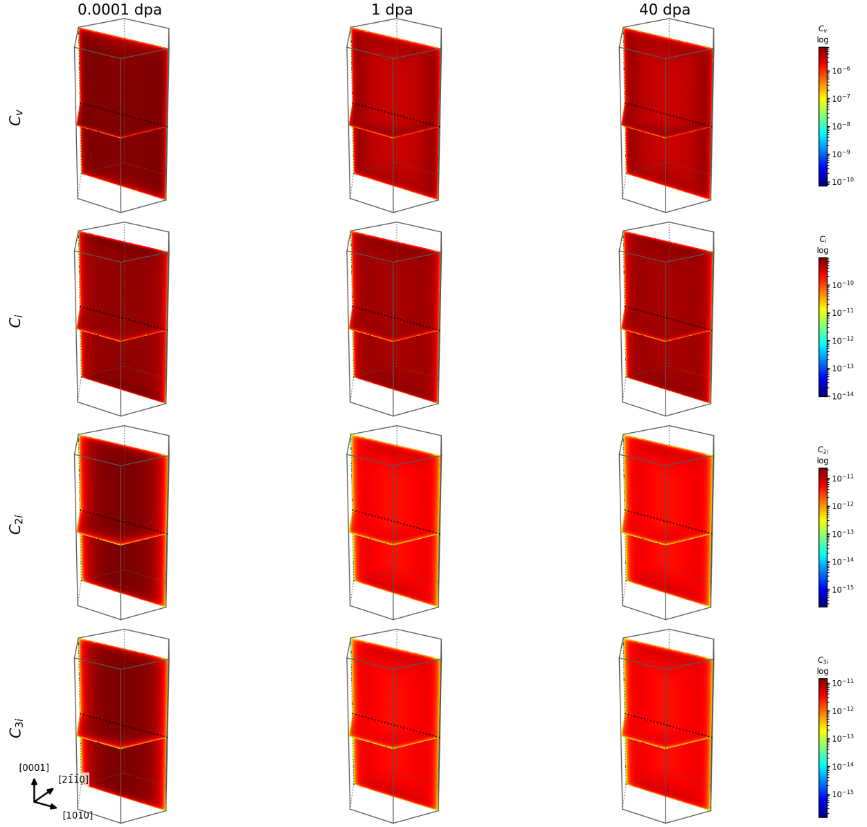
Figure 7: Mobile species at 10^{-4} , 1 and 40 dpa, on one vertical and one horizontal mid-cut. Rows, top to bottom: C_v , C_i , C_{2i} , C_{3i} ; each row has its own logarithmic color scale, so levels are comparable across dose within a row and not between rows. The middle column is where the evolution is visible: between 10^{-4} and 1 dpa the interior plateau falls and the depleted shell narrows, both because the sink density has risen, and between 1 and 40 dpa almost nothing further happens.
