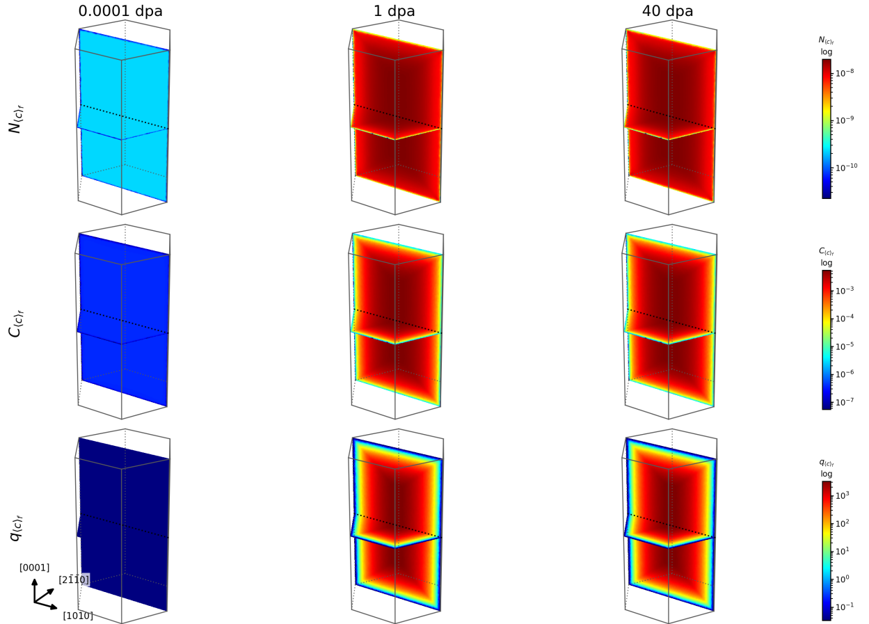
Figure 8: The basal faulted family c_f at 10^{-4} , 1 and 40 dpa: number density n (top), stored content c (middle), second content q (bottom).
