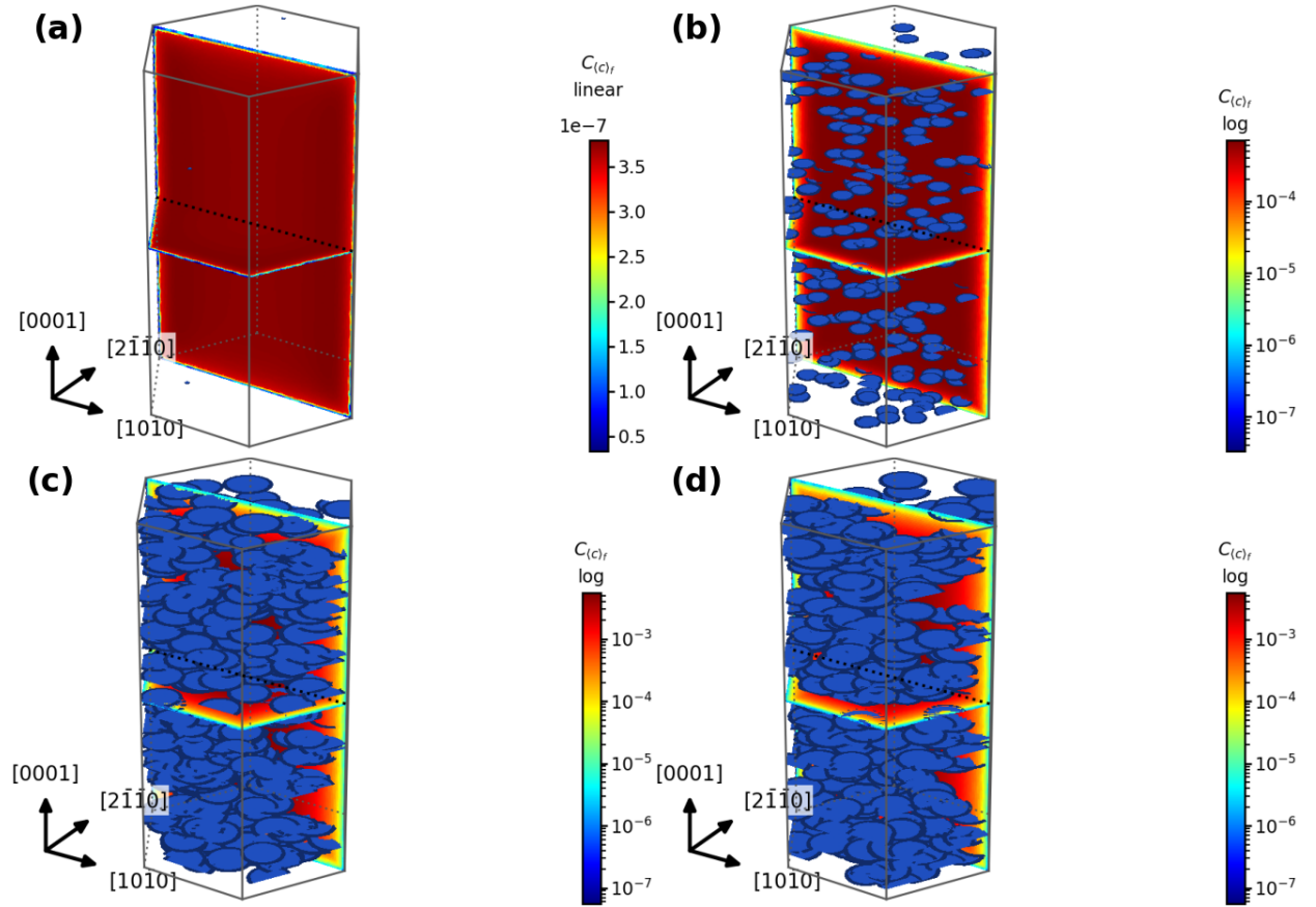
Figure 15: The discrete basal \langle c \rangle population at (a) 10^{-4} , (b) 10^{-2} , (c) 1 and (d) 40 dpa, at true radius and sampled position, drawn over the continuum field. The drawn loops are clipped at the crystal surface; the exported loops are whole.
