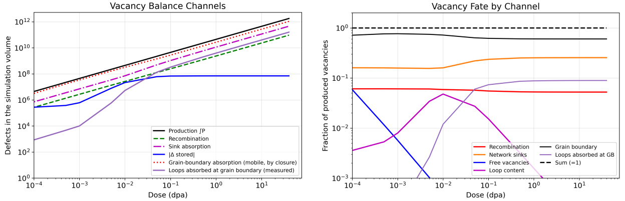
Figure 10: Vacancy balance against dose: cumulative channels (left) and their fractions of production (right). The interstitial counterparts are similar except that the loop-at-boundary channel is 709 times smaller.
