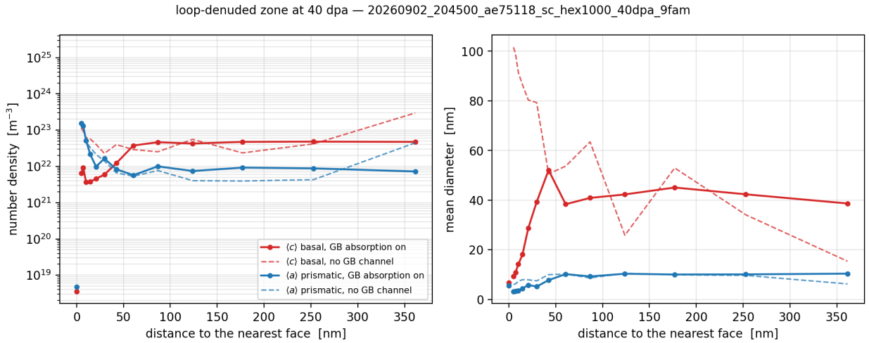
Figure 12: The loop-denuded zone at 40 dpa. Solid: grain-boundary loop absorption active. Dashed: the identical calculation without it. Left, number density; right, content-weighted mean diameter. The abscissa is the minimum distance to any face, and the ordinate on the left is logarithmic. This figure and the table below come from a companion pair on the same 1 \mu\text{m} geometry run at the uncalibrated parameter set, because the calculation reported elsewhere in this section has no matched twin without the channel; what the pair isolates is the channel, and the levels are not those of Table 9.
