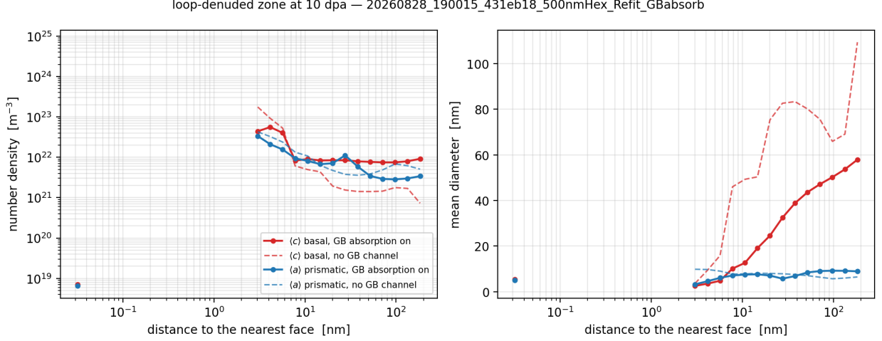
Figure 12: The loop-denuded zone at 10 dpa. Solid: grain-boundary loop absorption active. Dashed: the identical calculation without it. Left, number density; right, content-weighted mean diameter. The abscissa is the minimum distance to any face, and the ordinate on the left is logarithmic over six decades.
