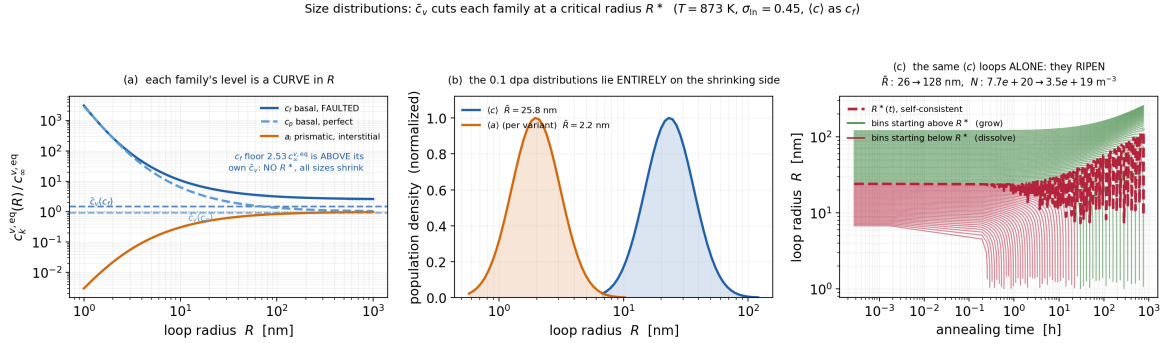
Figure 8: What a size distribution changes. (a) Each family’s level is a curve in R , drawn against the \bar{c}_v its own mixture produces; the dotted horizontals are the floors Eq. (194). The faulted basal state’s floor lies above its own \bar{c}_v , so Eq. (193) has no root. (b) The reference distributions at 0.1 dpa lie entirely on the shrinking side of \bar{c}_v . (c) The same \langle c \rangle population with the network and the \langle a \rangle loops removed, so that \bar{c}_v is its own: every size bin’s trajectory, with the self-consistent R^*(t) drawn through them. Bins that start above R^* grow at the expense of those below, which is ripening and not annealing. The sawtooth on R^*(t) is the bin discretization — \bar{c}_v is a sum over delta functions, so every bin that dissolves steps it — and not a feature of the solution. The distribution width \sigma_{ln} = 0.45 is the one assumed quantity in this figure. Produced by ...loop_annealing_population figure-ripening .
