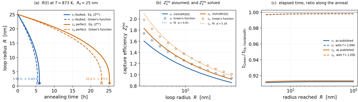
Figure 4: Figure 3(a) repeated with the boundary-integral solution superimposed. (a) R(t) at 873 K from R_0 = 25 nm: solid is Eq. (180) with Eq. (179), dashed the same law with Z solved from Eq. (182). (b) Z_k^{\text{iso}} assumed against Z_k^{\text{iso}} solved, with the one-parameter refit of Table 12. (c) The elapsed-time ratio along the anneal, before and after the constant refit f — it is flat, which is the statement of item 1 above, and f removes it to 0.2%. Produced by disloccluster_code.studies.loop_annealing_greens figure-rt .
