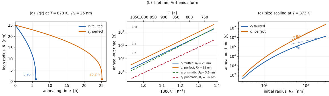
Figure 3: Thermal anneal of an isolated basal vacancy loop from Eq. (180), for the faulted state c_f and the perfect state c_p of Table 2. (a) R(t) at 873 K from R_0 = 25 nm, on a linear time axis: the faulted loop reaches the floor in 5.95 h and the perfect one in 25.2 h, and the two curves have different shapes and not merely different rates. (b) The anneal-out time in Arrhenius form, with the two prismatic families added at their own reference size R_0 = 3.6 nm; the slopes give Q_{\text{eff}} = 2.56\text{--}2.79 eV against E_v^f + E_v^m = 2.80 eV. (c) The size dependence at 873 K, with the two asymptotes of Eq. (181) drawn as guides. Produced by disloccluster_code.studies.loop_annealing figure .
