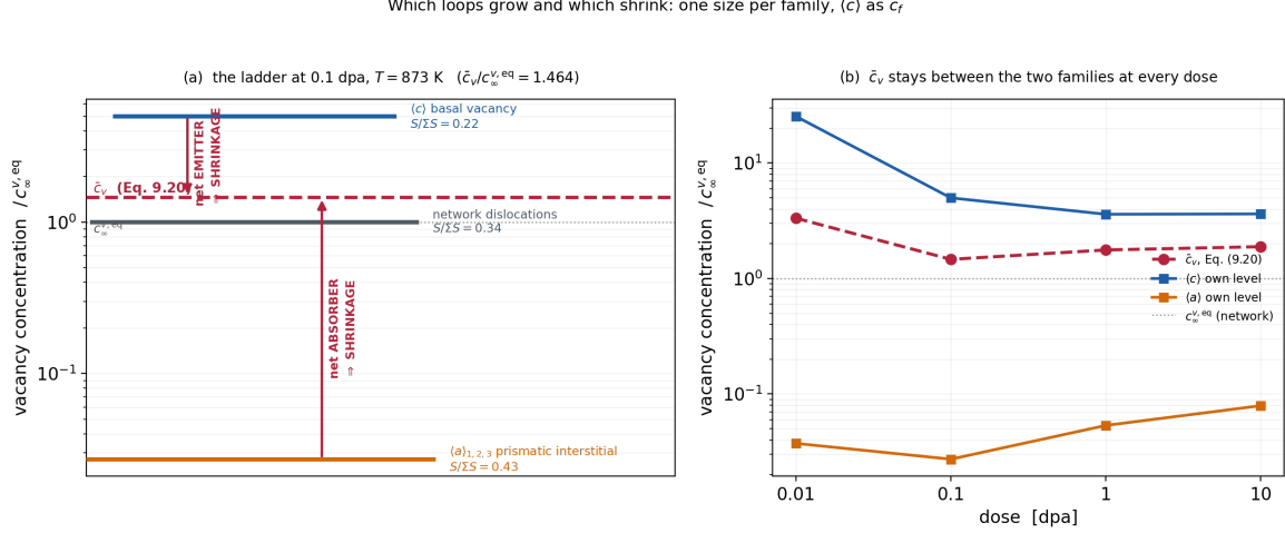
Figure 6: The concentration ladder of Eq. (190), one size per family, on the interior state of the reference march at 873 K. (a) Each rung is a component's own c_k^{v,\text{eq}} and its width is that component's weight S_k / \sum S_k in Eq. (190); the dashed line is the solved \bar{c}_v . The \langle c \rangle loops are net emitters and the \langle a \rangle loops net absorbers, and both shrink, because s_s(v) has opposite signs for them. (b) The same across dose: \bar{c}_v tracks between the two families at every one, never leaving the interval the rungs bracket. Produced by dislocluster_code.studies.loop_annealing_population figure-ladder .
