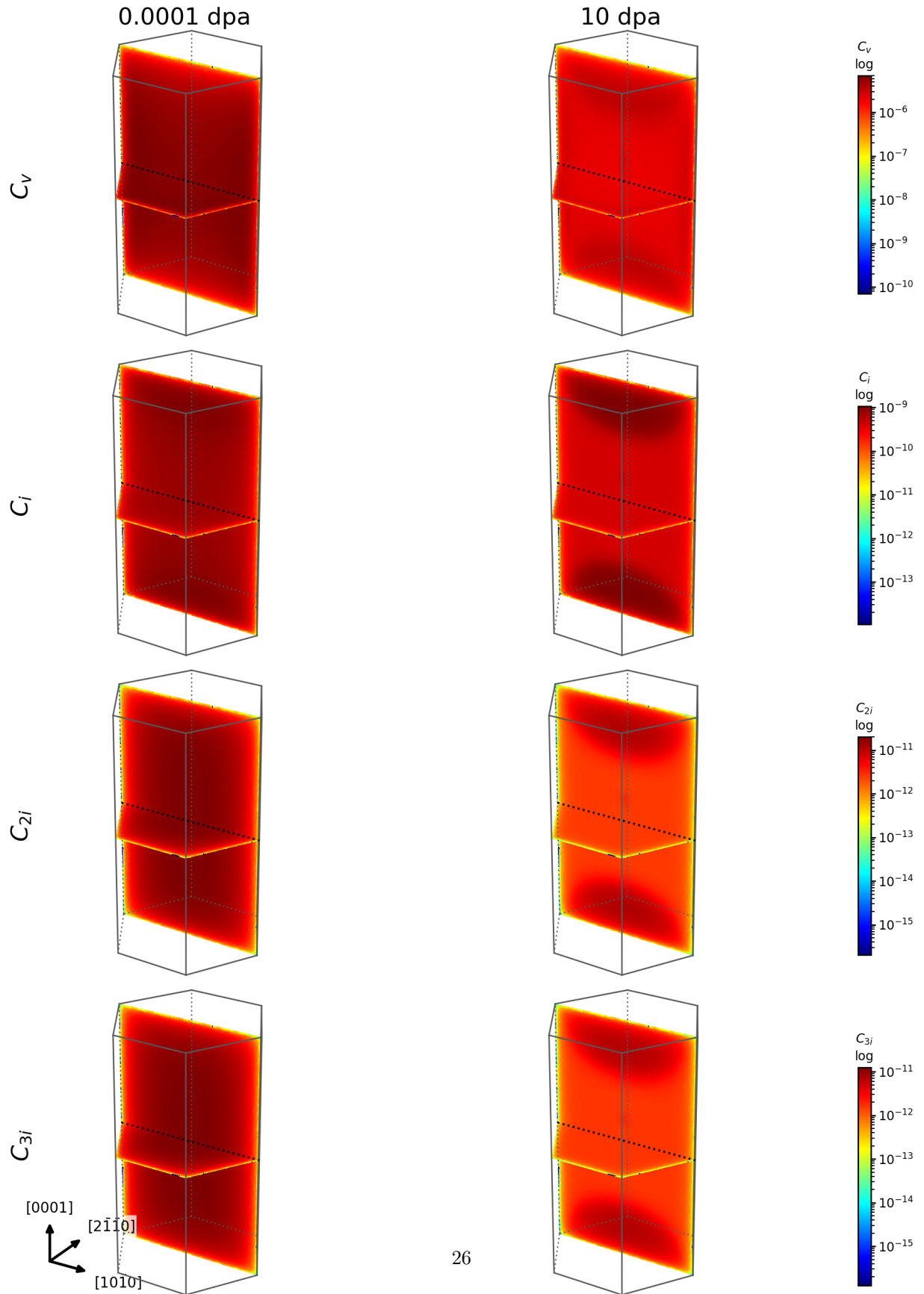
Figure 7: Mobile species at 10^{-4} dpa (left) and 10 dpa (right), on one vertical and one horizontal mid-cut. Rows, top to bottom: C_v , C_i , C_{2i} , C_{3i} ; each row has its own logarithmic color scale, so levels are comparable across dose within a row and not between rows. The interior plateau falls and the depleted shell narrows between the two doses, both because the sink density has risen.
