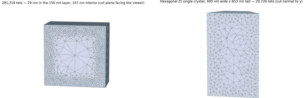
Figure 28: Mesh-dependence studies. Left: cubic verification domain, 281,218 tetrahedra, graded from 29 nm in the 150 nm boundary layer to 147 nm in the interior (cut plane facing the viewer). Right: hexagonal Zr single crystal, 400 nm wide by 653 nm tall, 20,726 tetrahedra (cut normal to y ).
