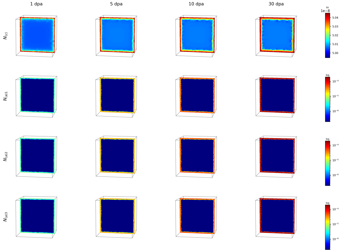
Figure 20: Loop number density for the basal \langle c \rangle family and the three prismatic \langle a \rangle families. At zero applied stress the three \langle a \rangle panels must be identical, and are; this is a check on the crystallography. Note the accumulation adjacent to the grain boundary.
