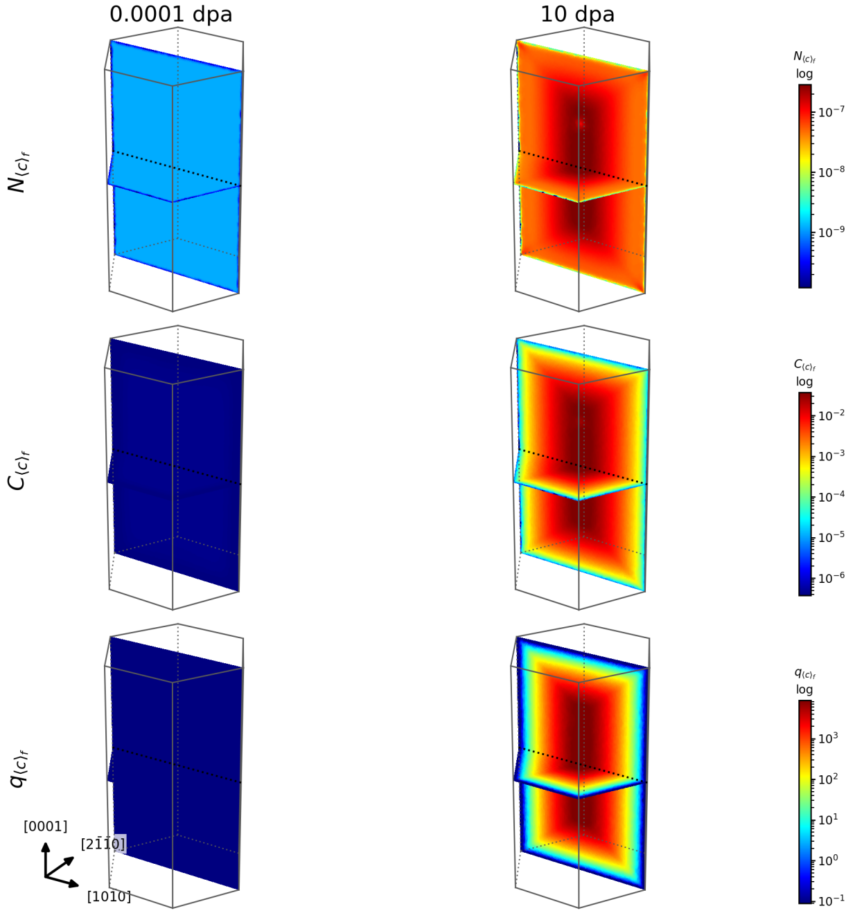
Figure 8: The basal faulted family c_f at 10^{-4} and 10 dpa: number density n (top), stored content c (middle), second content q (bottom).
