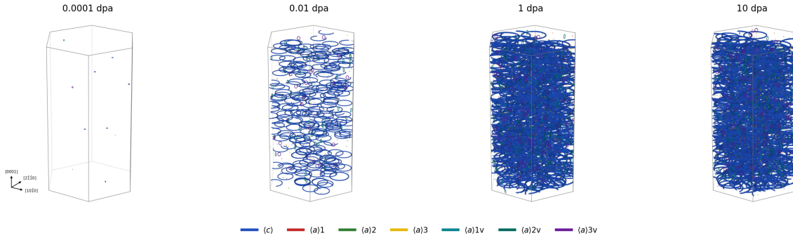
Figure 19: The discrete loop population of the interior at 10^{-4} , 10^{-2} , 1 and 10 dpa, every variant superimposed and drawn at its true radius and sampled position: basal \langle c \rangle in blue, the three interstitial prismatic variants in red, green and gold, and the three vacancy prismatic variants in teal and purple. Each panel is the same crystal and the same viewpoint, so the panels are comparable across dose. The interior population runs 55 \rightarrow 333 \rightarrow 882 \rightarrow 1414 loops over the four panels, and the basal share of it 13\% \rightarrow 50\% \rightarrow 45\% \rightarrow 43\% — so what the sequence shows is not the basal family becoming more numerous but its loops becoming very much larger, until at 10 dpa they dominate the drawing at a diameter an order of magnitude above the prismatic variants. The three interstitial prismatic variants stay exactly equal in number (202 each at 10 dpa), which is the isotropic variant weighting of Eq. (34) under zero applied stress; the three vacancy variants likewise (65 each). That domination by size is why Figs. 15 and 16 separate the families; here it is the subject.
