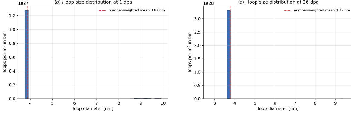
Figure 29: \langle a \rangle_3 loop size distributions at 1 dpa (left) and 26 dpa (right). The number-weighted mean diameter is nearly dose-independent while the number density grows by more than an order of magnitude, the signature of a nucleation-dominated population.
