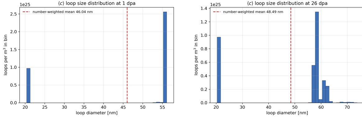
Figure 30: \langle c \rangle loop size distributions at 1 dpa (left) and 26 dpa (right). The interior population coarsens slowly with dose while a stationary near-boundary population remains near 20 nm; the number-weighted mean moves from 46.0 to 48.5 nm.
