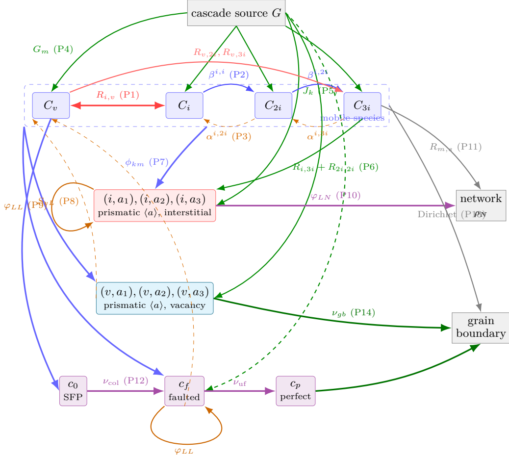
Figure 2: Reaction admissibility graph for the nine families of Eq. (3), with every edge class of Table 2. The four mobile species are boxed together because capture onto a loop sums over all of them (Eq. (29)), with a sign set by whether the species' polarity matches the family's, so one bundled arrow per family is faithful where four would be unreadable. Cascade production (green) feeds all four mobile species and, as a separate partition of the same displacement rate, nucleates the prismatic loops of both characters and the basal family directly; the dashed source onto c_f becomes a source onto c_0 instead when the basal chain is active, which it is not in Section 7. The interstitial prismatic family has a second, homogeneous nucleation channel (P6) fed by 2i + 2i and i + 3i reactions among the mobile clusters, which is why the mobile ladder and the loop populations are not separable. Dashed orange edges run backwards from a population to the mobile pool: dissociation of a small cluster (P3) and peripheral emission from a vacancy loop (P8). The three prismatic variants of each character are drawn as one vertex for legibility; they are separate populations that exchange nothing with one another and differ only in habit normal, and the pyramid c_0 is not a loop — it has no Burgers vector, no perimeter and no coalescence channel, and enters only through a capture cross-section.
