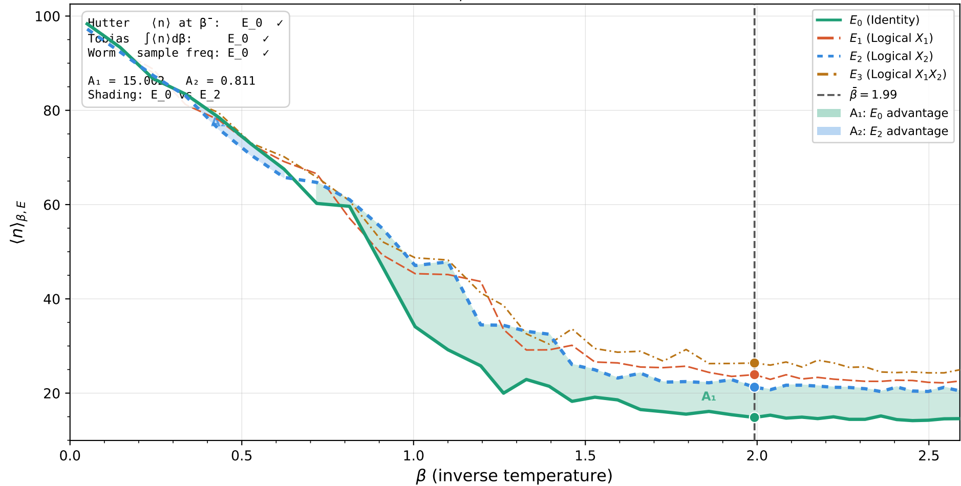
Toric code — \langle n \rangle_{\beta, E} curves ( L = 10 , p = 0.12 )
