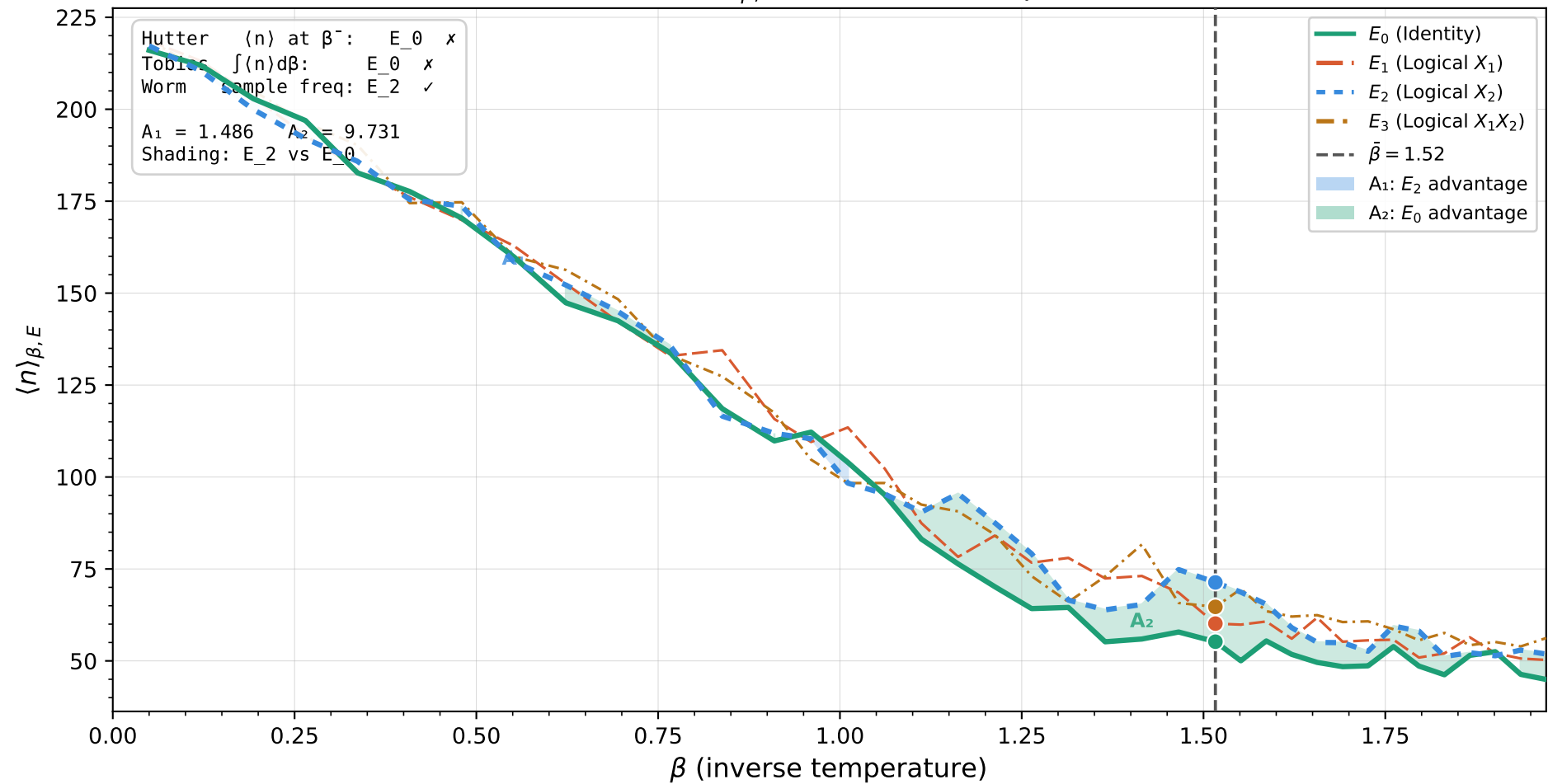
Toric code — \langle n \rangle_{\beta, E} curves ( L = 15 , p = 0.18 )
