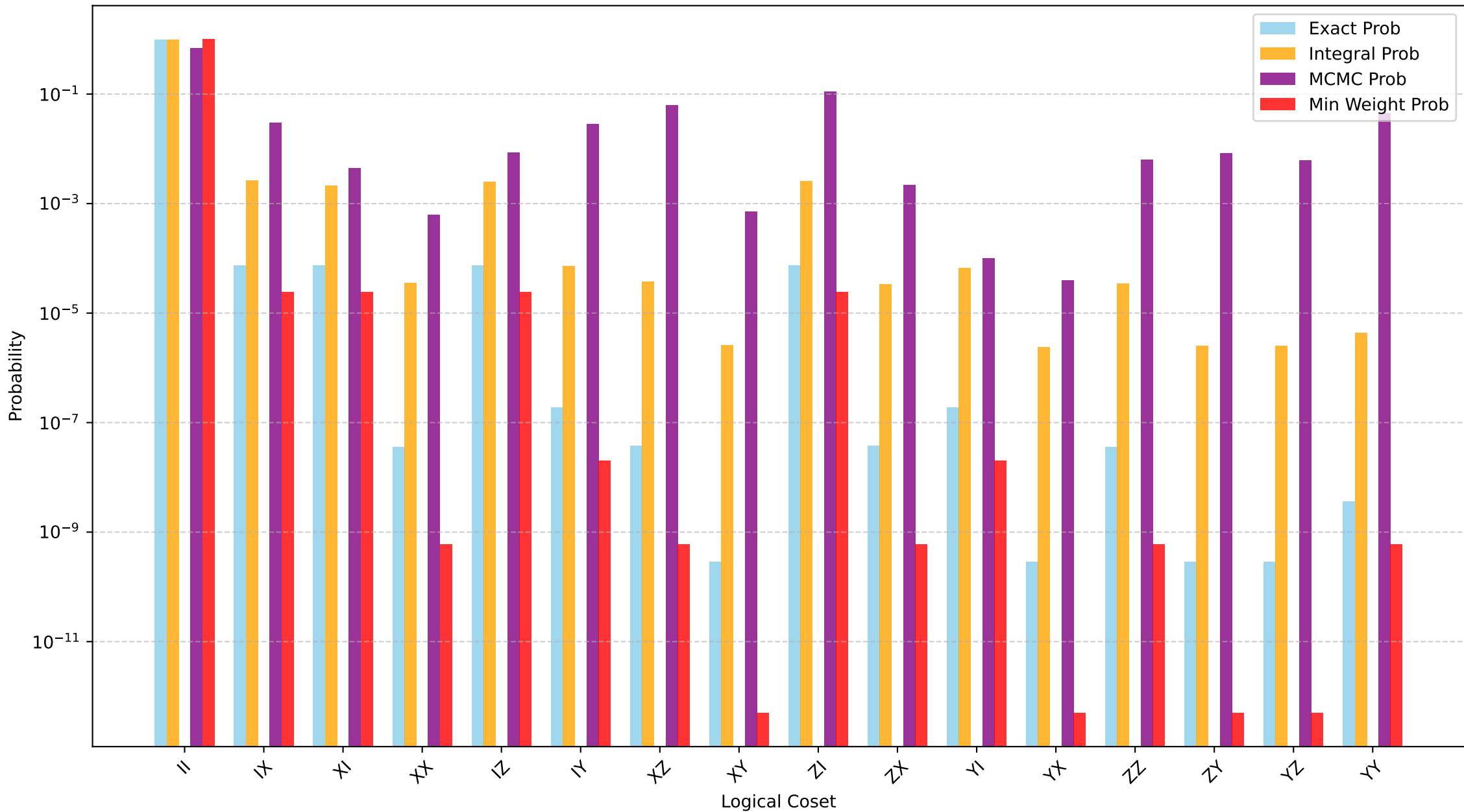
Coset Probabilities Proxies Comparison (L=3, p=0.08)
