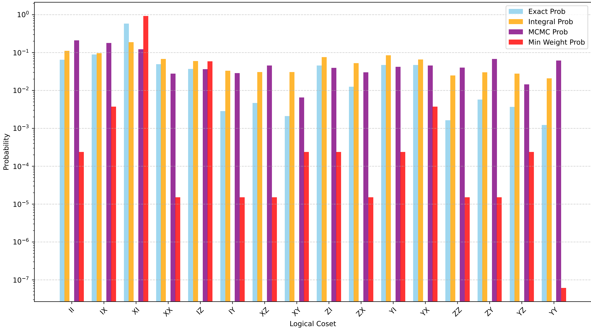
Coset Probabilities Proxies Comparison (L=3, p=0.16)
